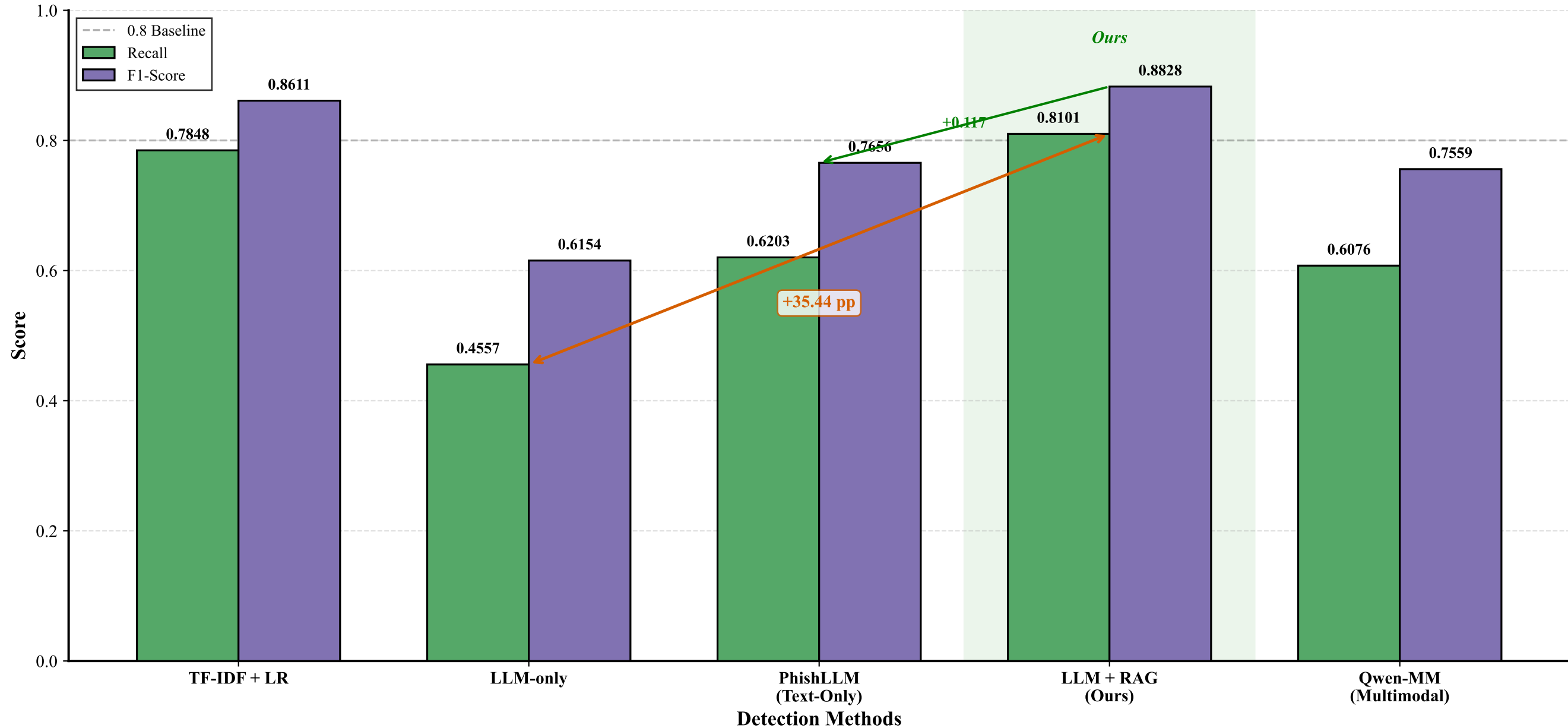
Figure 2: Recall and F1-Score Comparison (Core Metrics)
