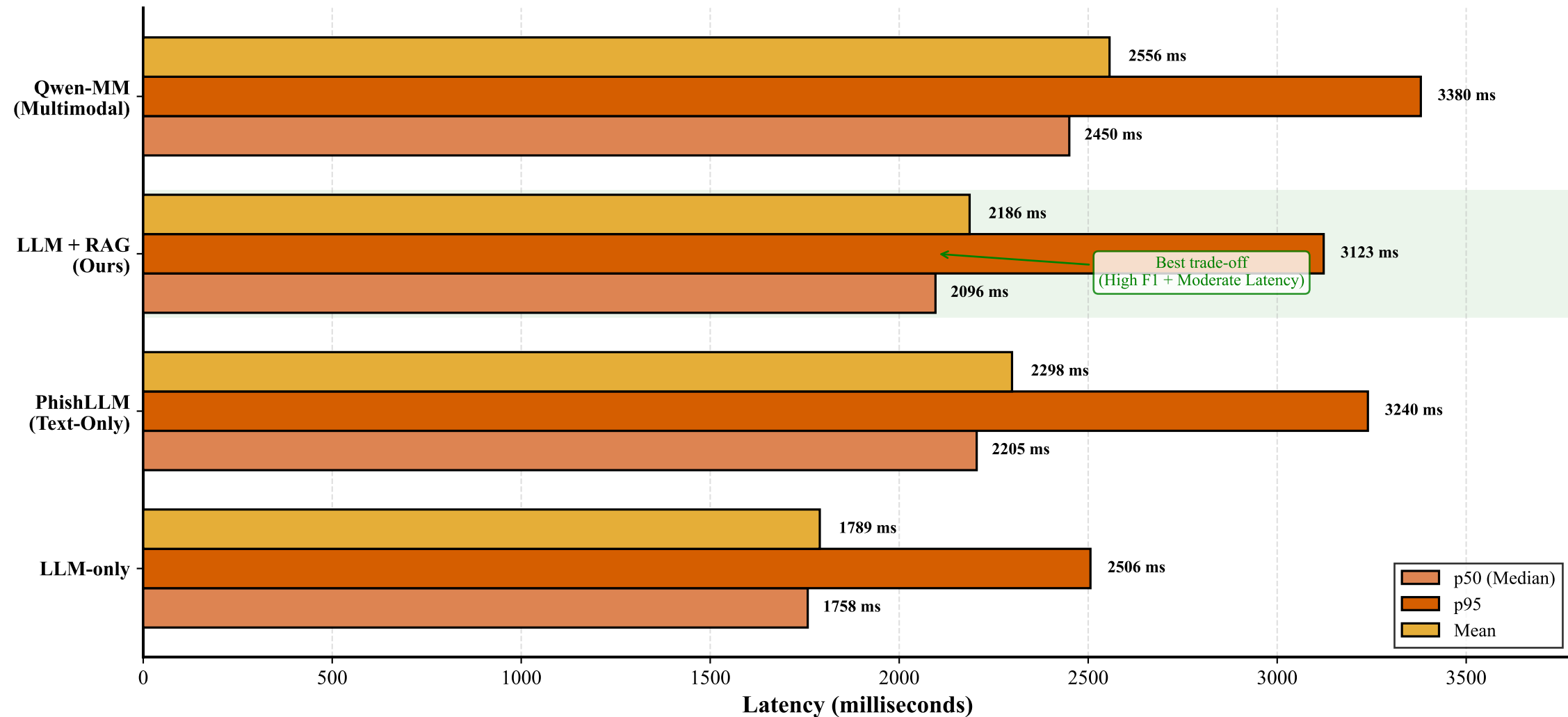
Figure 3: Inference Latency Comparison
