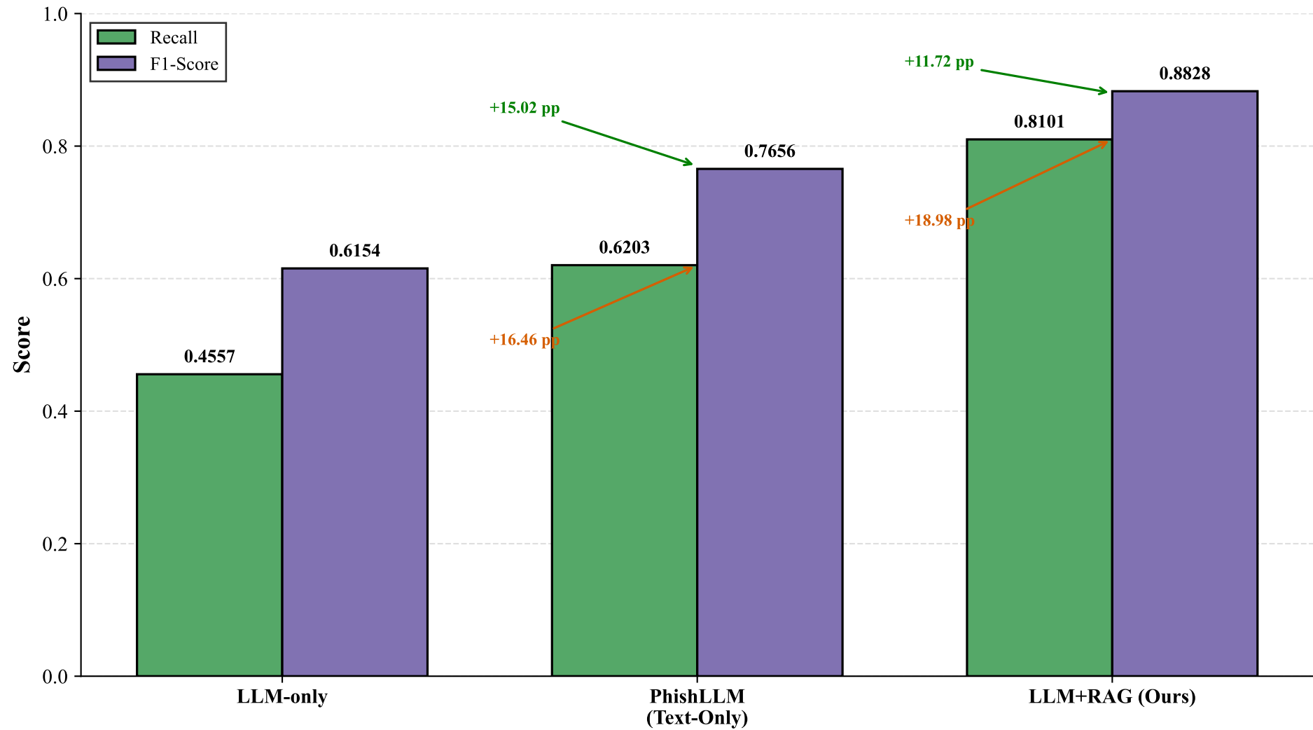
Figure 5: Text-Only Methods Progressive Improvement
