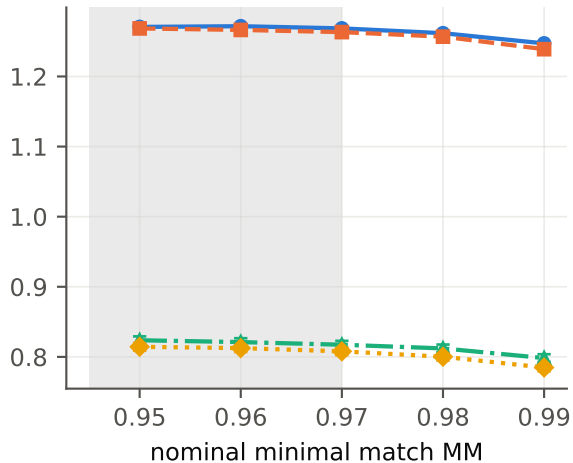
IMRPhenomD — declared approximation
