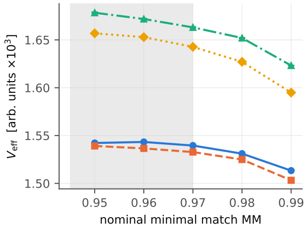
TaylorF2 — discretisation only
