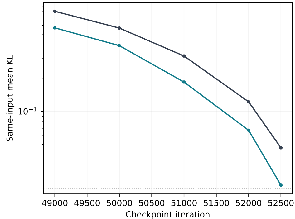
Pure student vs fused policy
