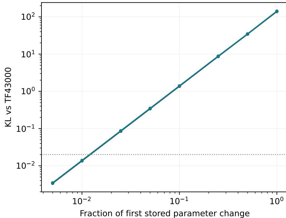
Stored update interpolation (not retraining)
