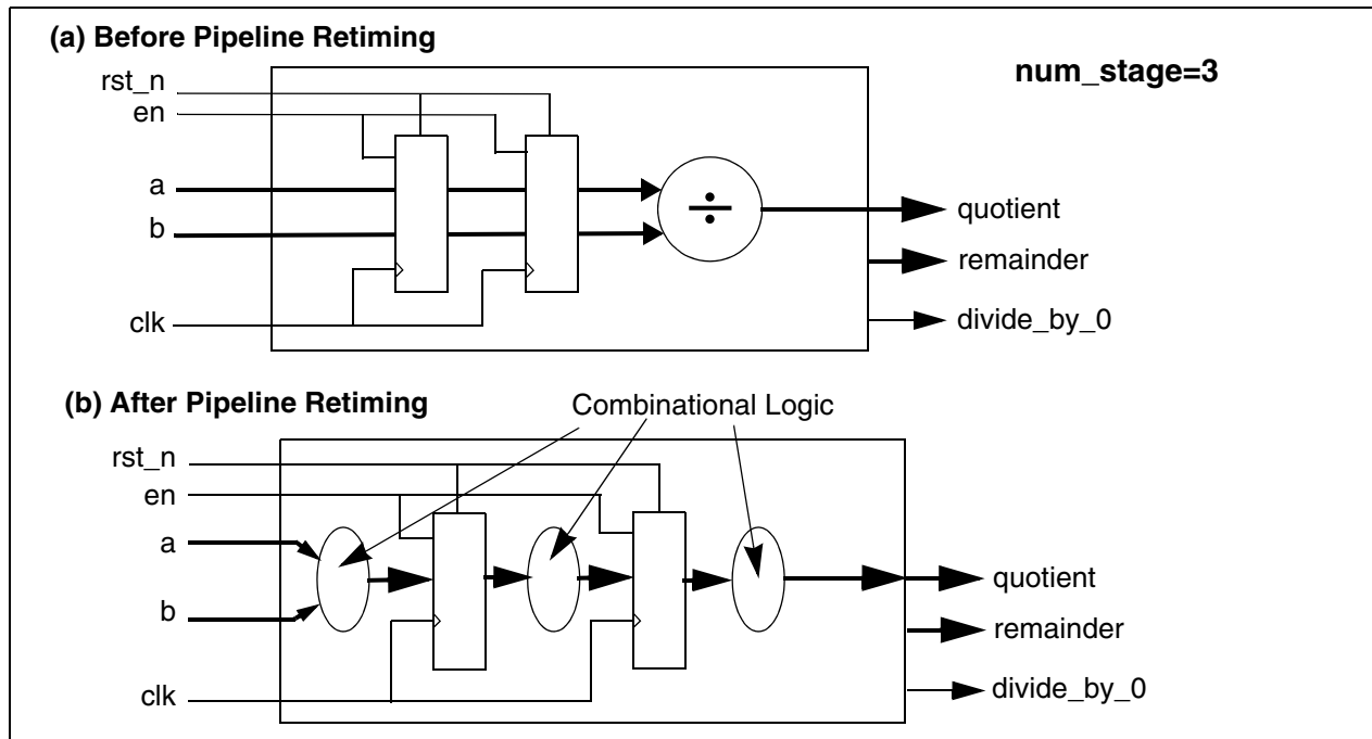
Figure 1-1 Pipeline Retiming
