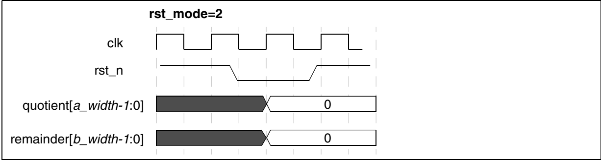
Figure 1-5 Waveform 4
