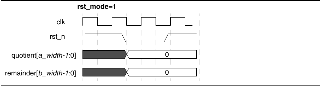
Figure 1-5 Waveform 4
