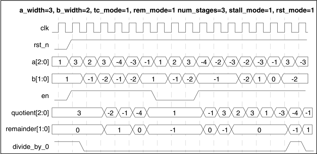
Figure 1-4 Waveform 3
