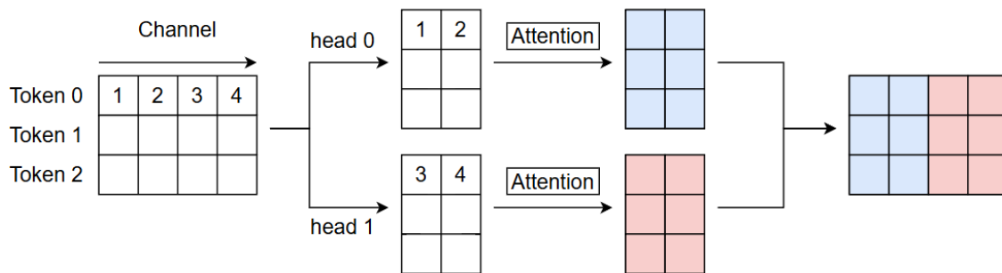
Fig. 8 Multi-head Self-Attention
