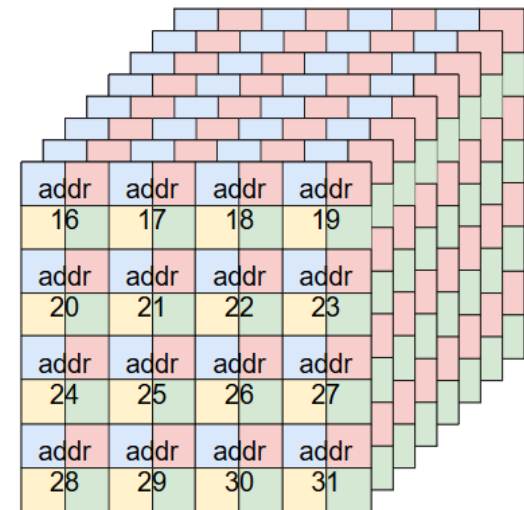
Head 1
