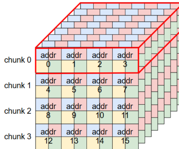
Head 0
