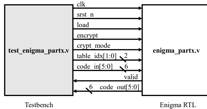
Fig. 13. System diagram
