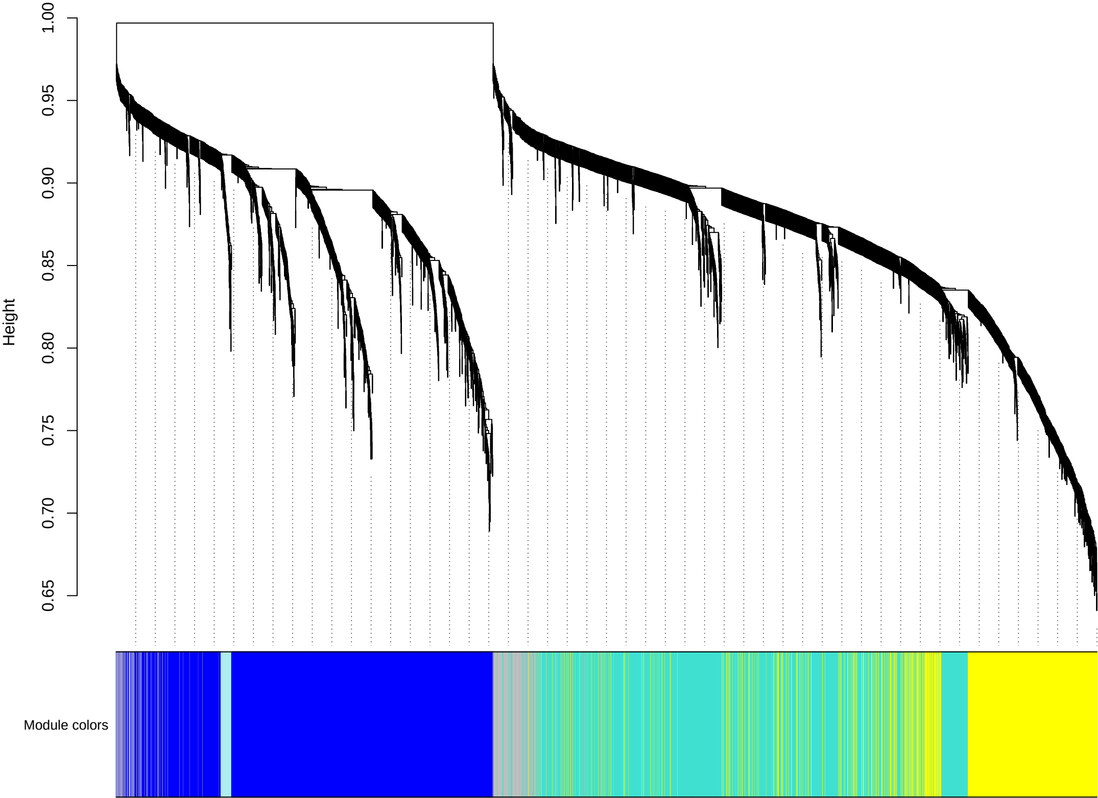
Gene dendrogram and module colors – Block 1
