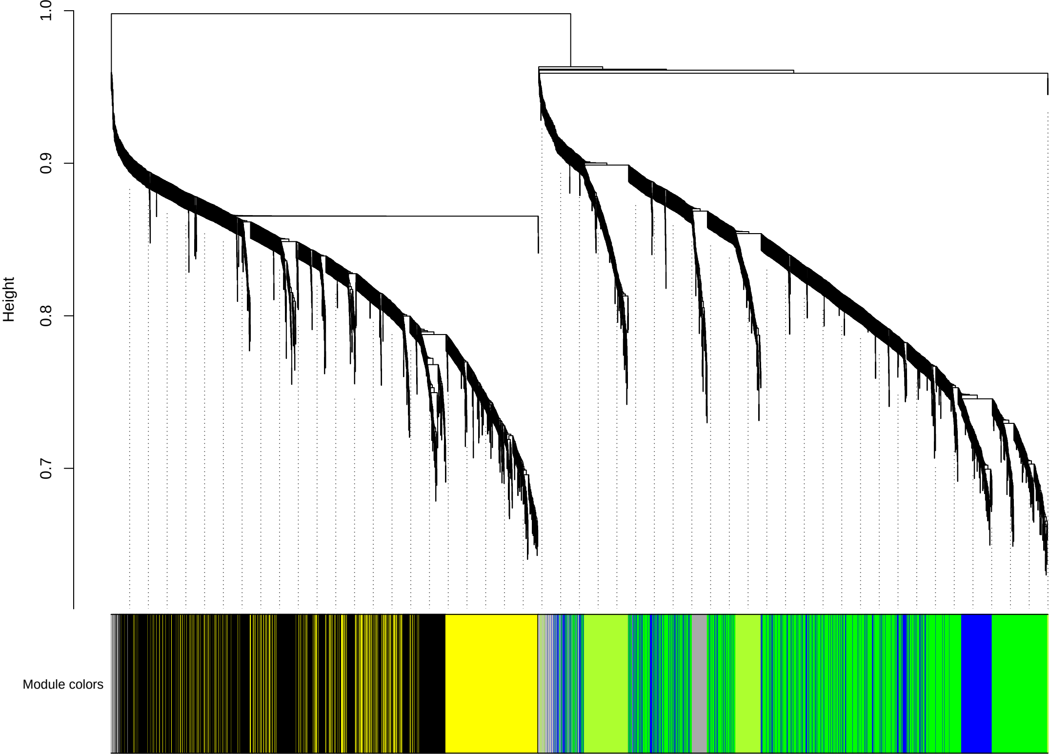
Gene dendrogram and module colors – Block 6
