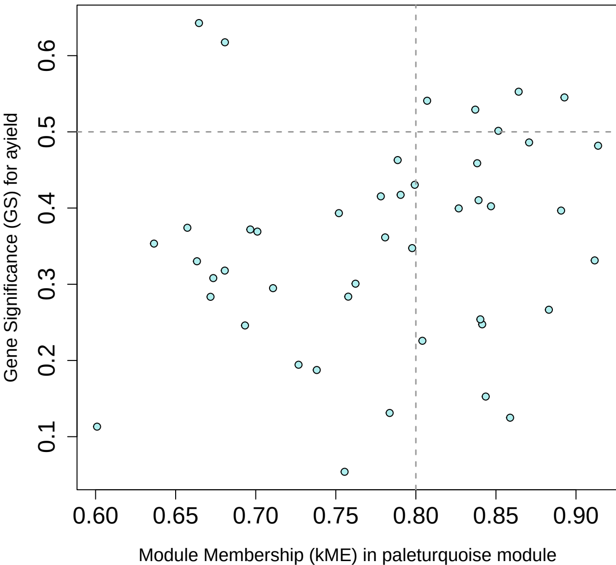
Membership vs. Significance paleturquoise module cor=0.18, p=0.24
