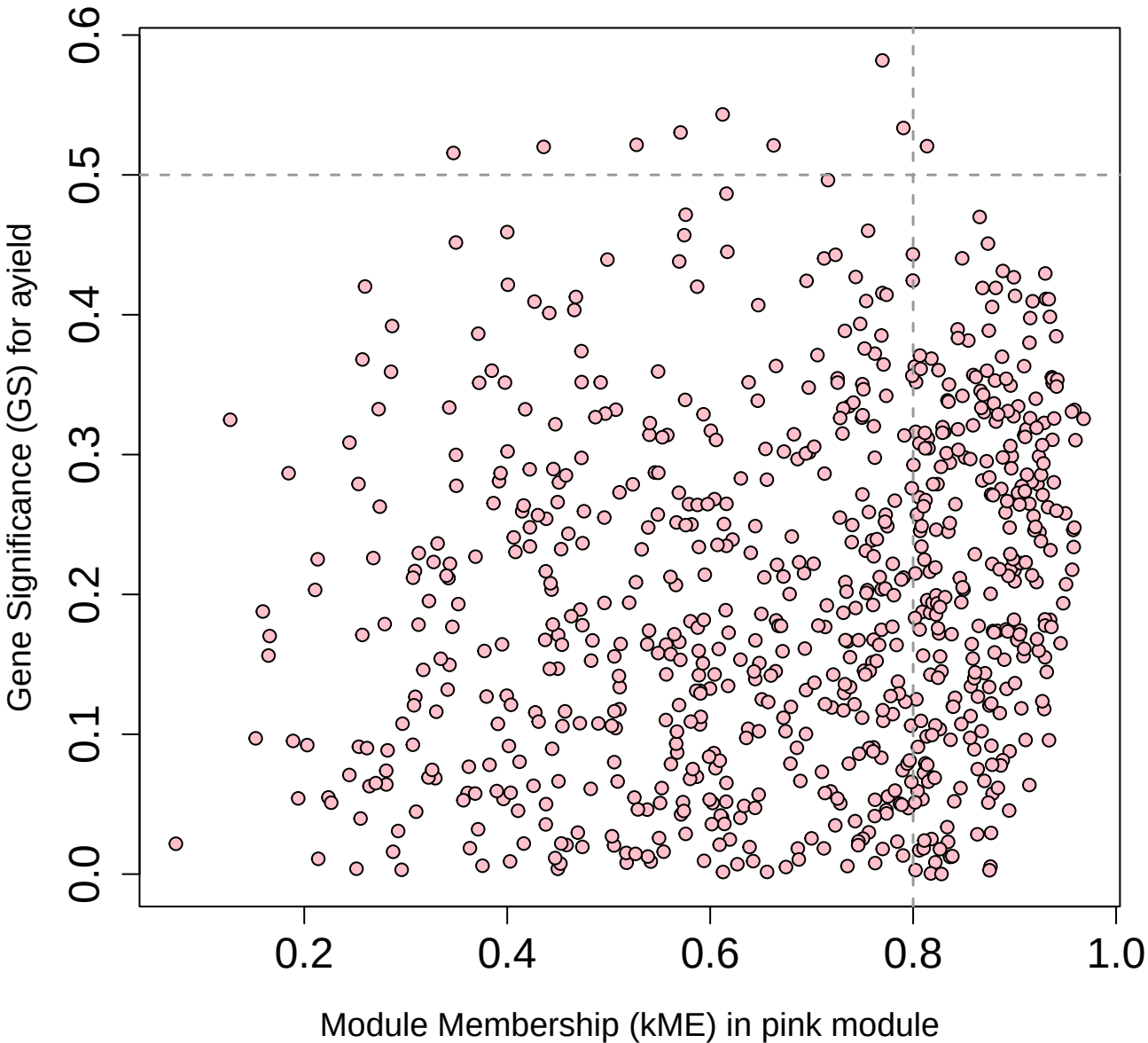
Membership vs. Significance pink module cor=0.17, p=2e-06
