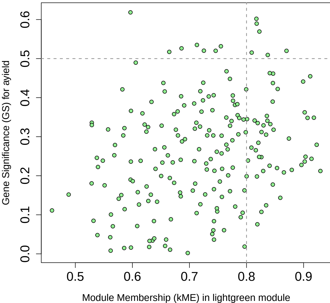
Membership vs. Significance lightgreen module cor=0.29, p=3.1e-05
