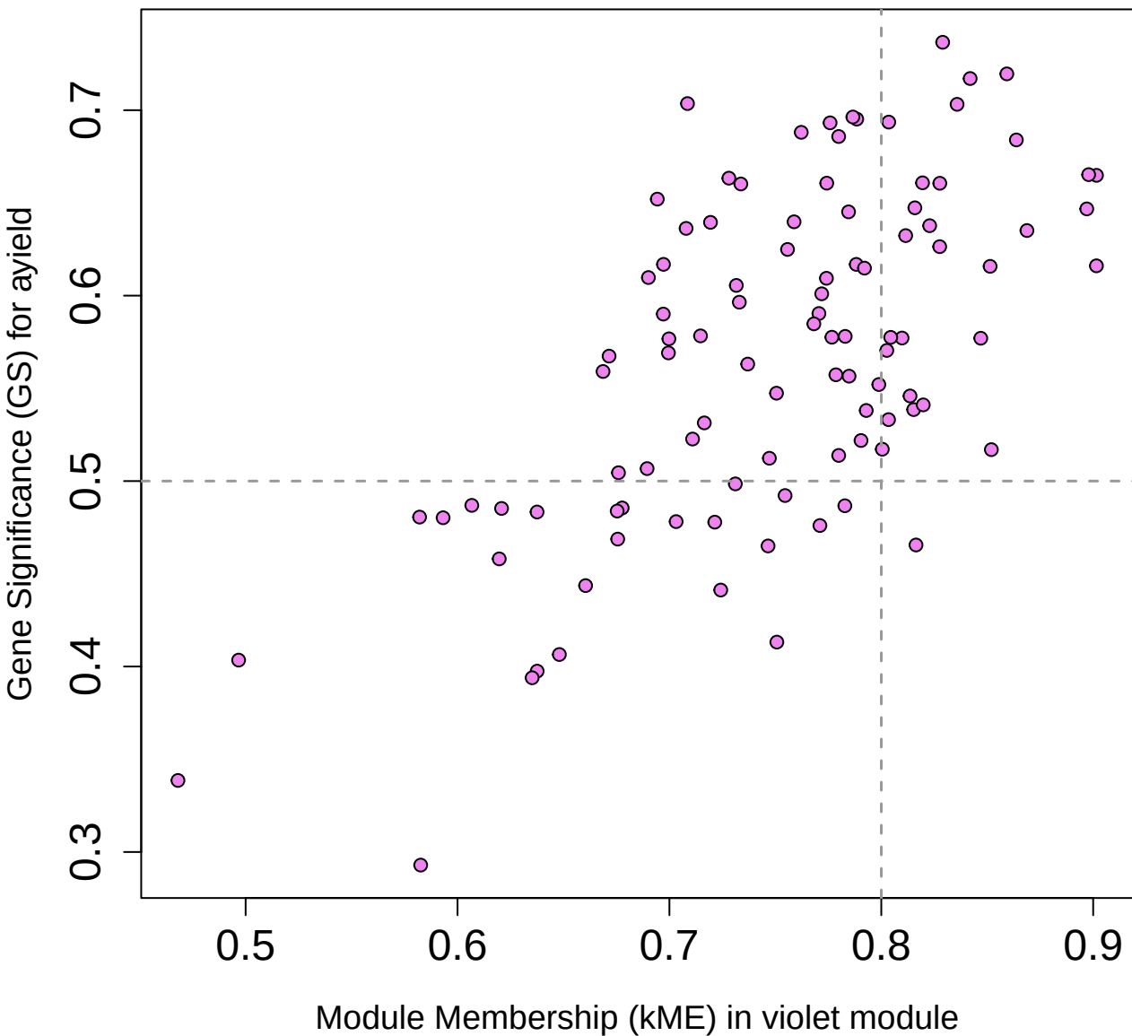
Membership vs. Significance violet module cor=0.64, p=7.6e-13
