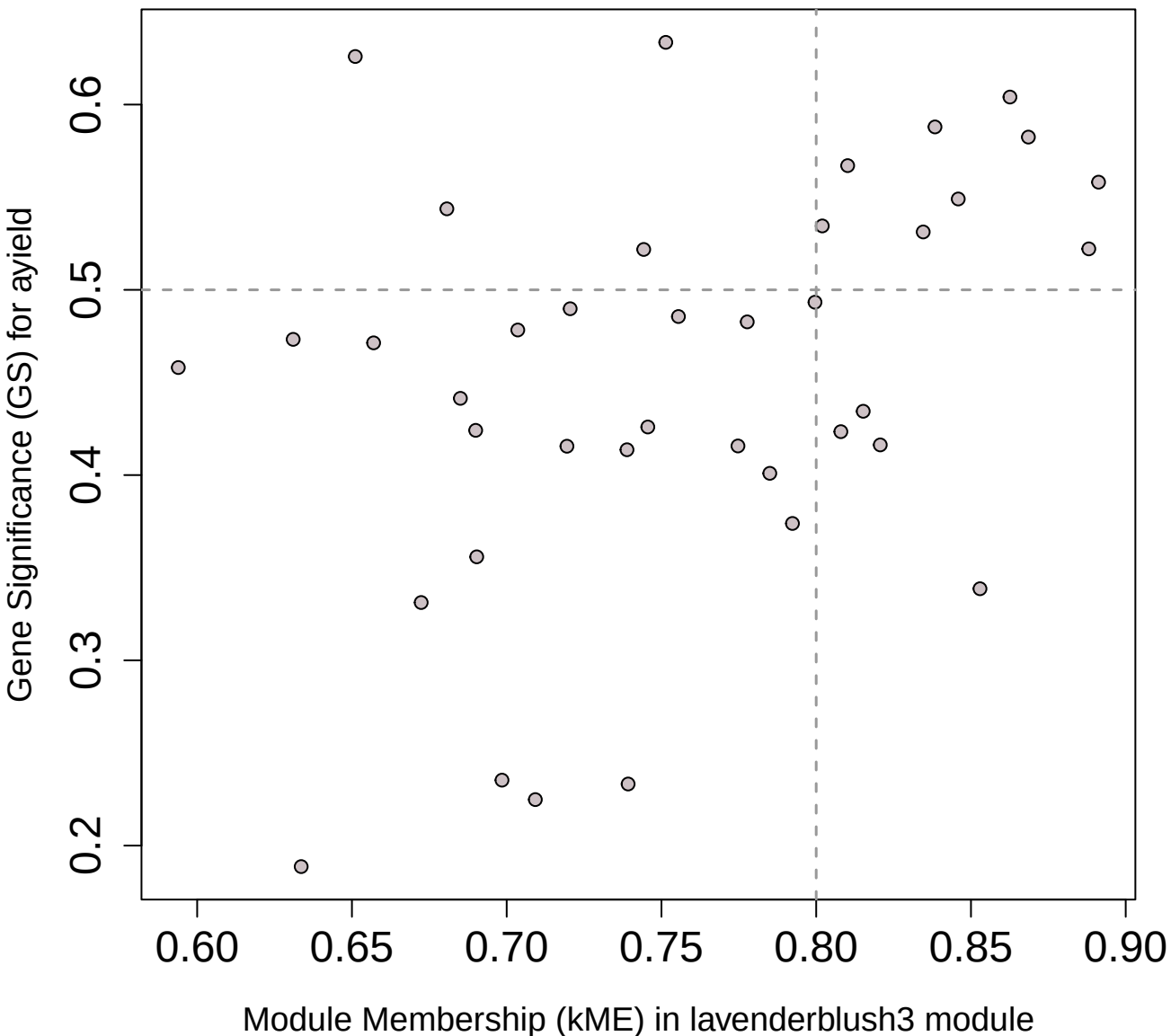
Membership vs. Significance lavenderblush3 module cor=0.36, p=0.024
