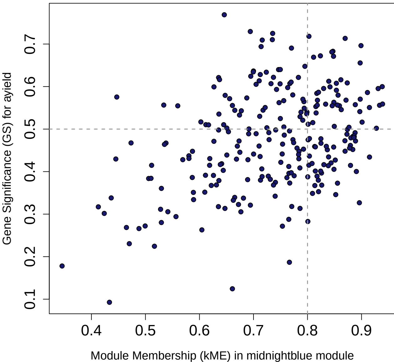
Membership vs. Significance midnightblue module cor=0.39, p=1e-10
