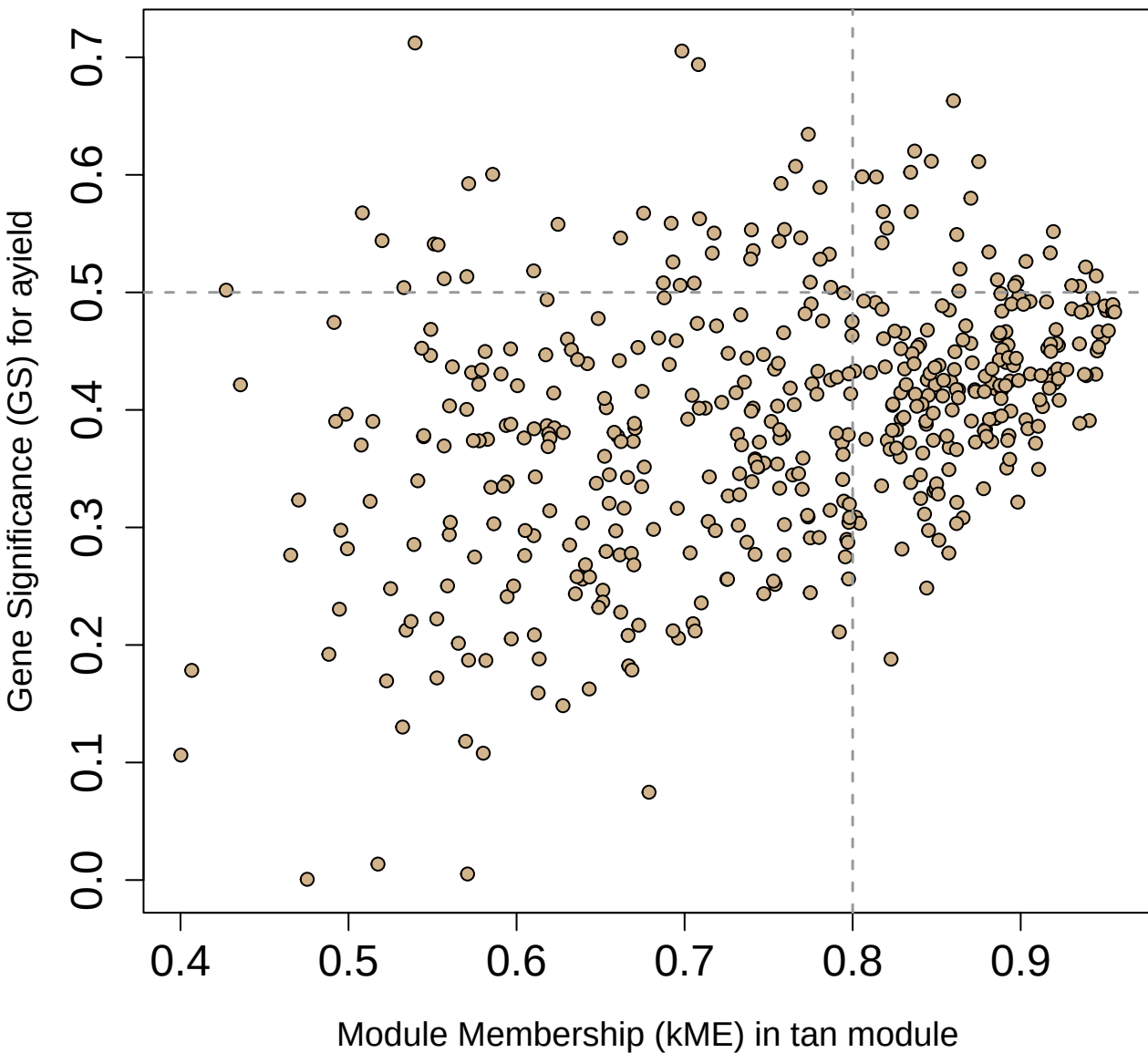
Membership vs. Significance tan module cor=0.36, p=9.1e-16
