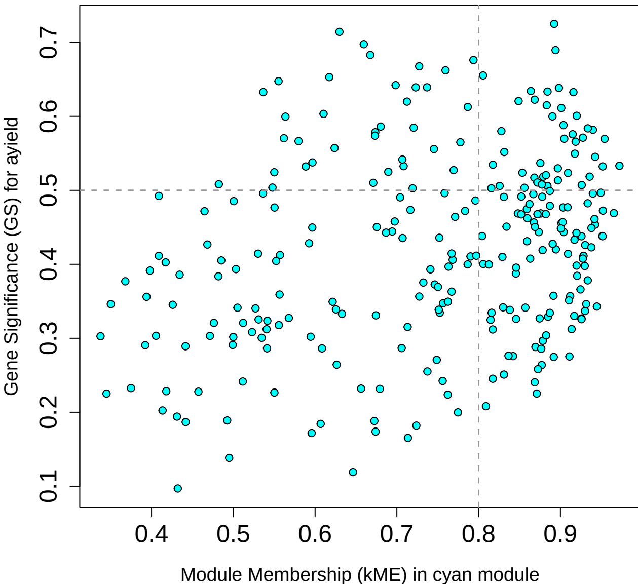
Membership vs. Significance cyan module cor=0.3, p=3.4e-07
