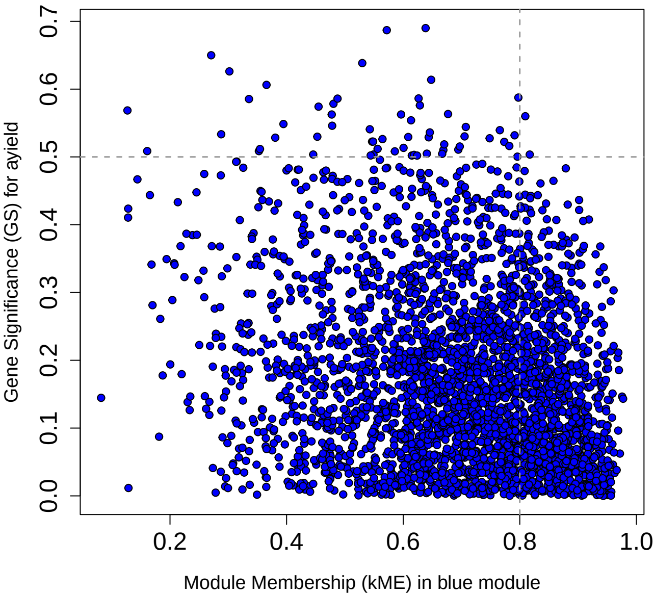
Membership vs. Significance blue module cor=-0.23, p=2.8e-39
