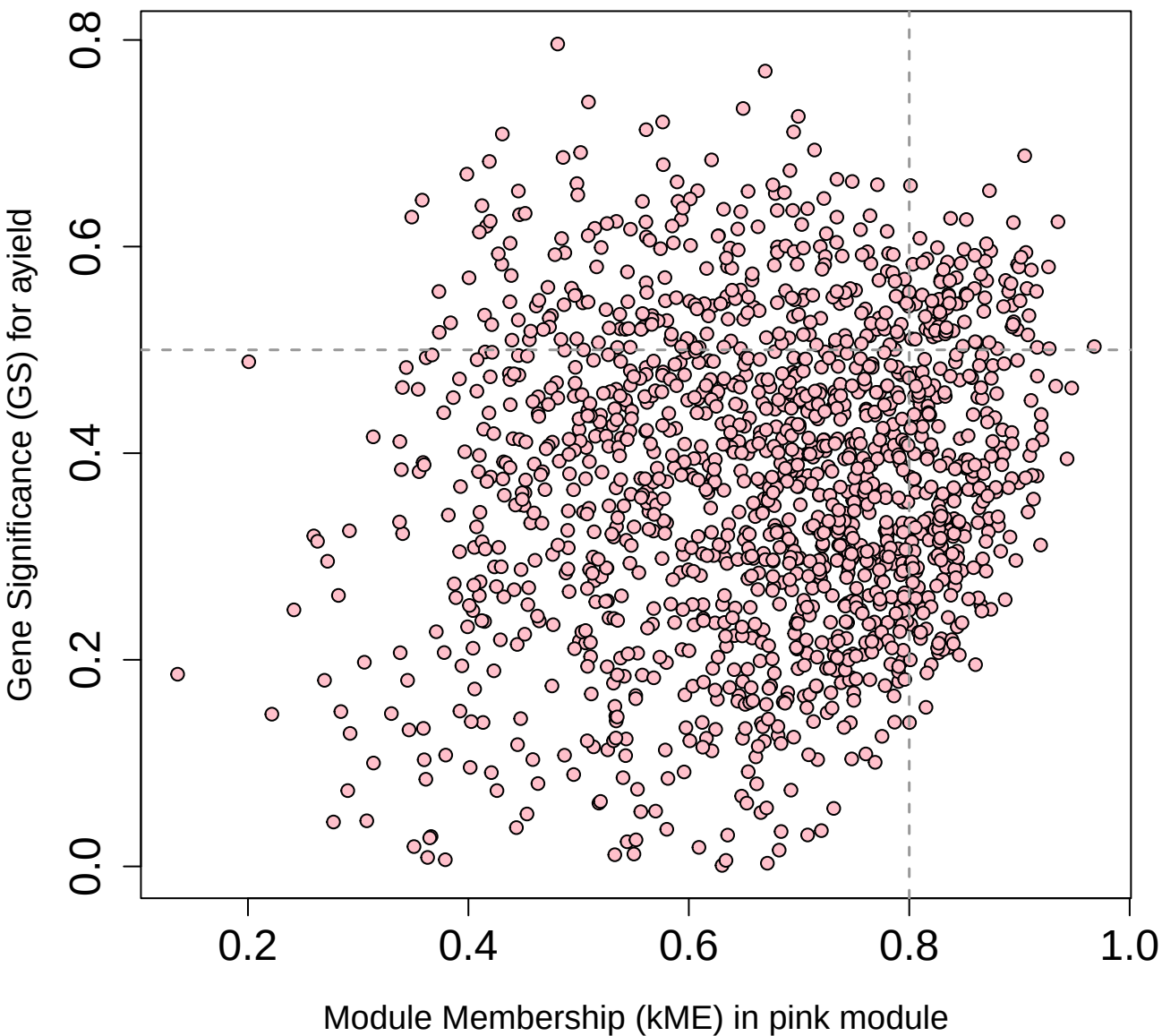
Membership vs. Significance pink module cor=0.12, p=2.8e-06
