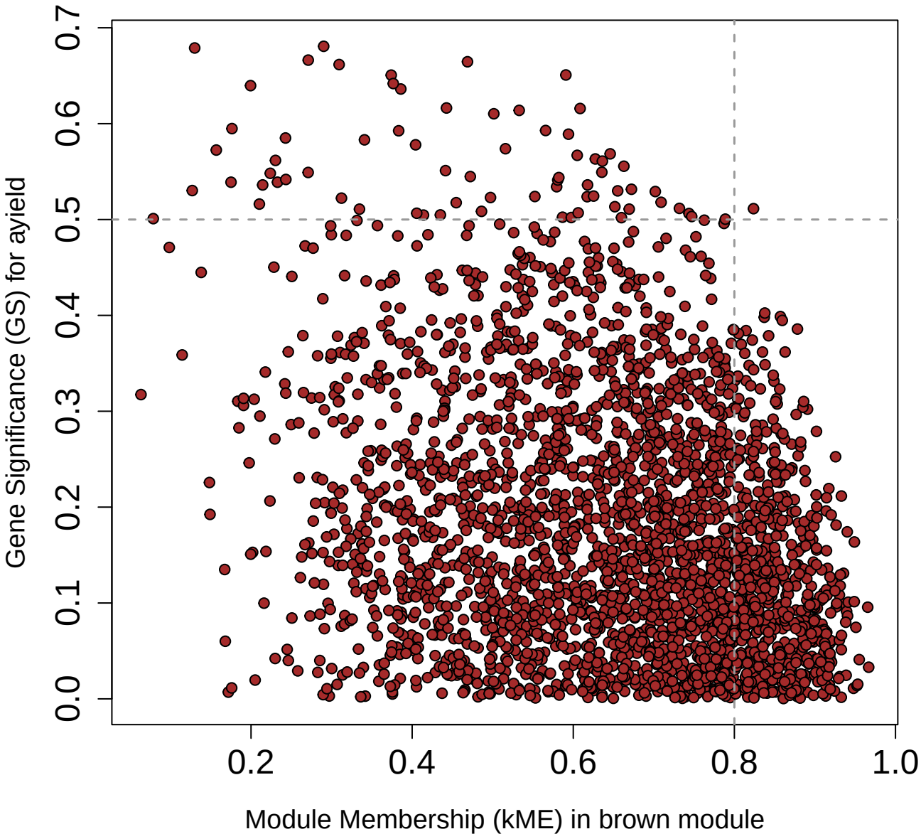
Membership vs. Significance brown module cor=-0.28, p=1e-51
