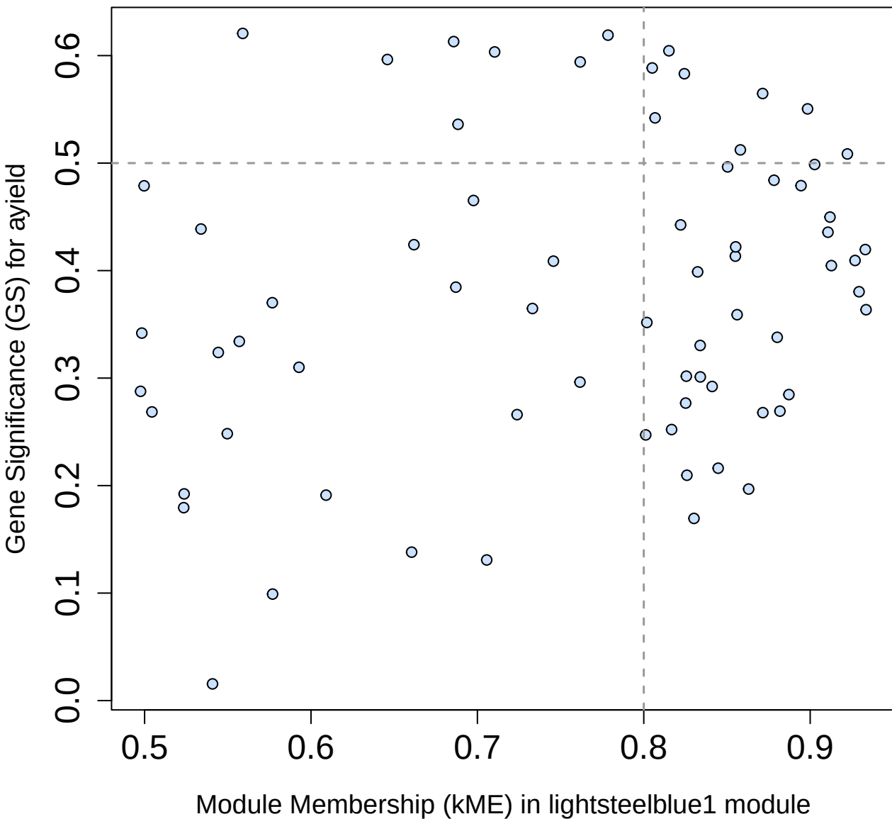
Membership vs. Significance lightsteelblue1 module cor=0.24, p=0.044
