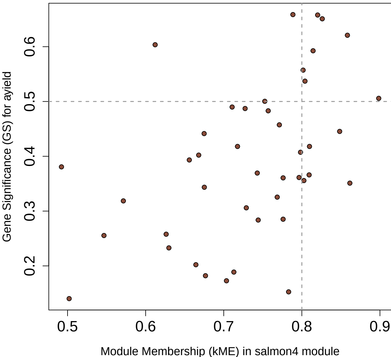
Membership vs. Significance salmon4 module cor=0.46, p=0.0019
