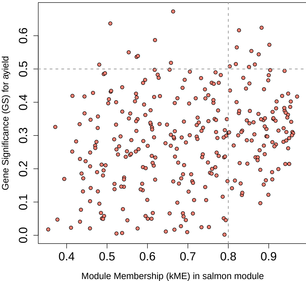
Membership vs. Significance salmon module cor=0.22, p=9.4e-05
