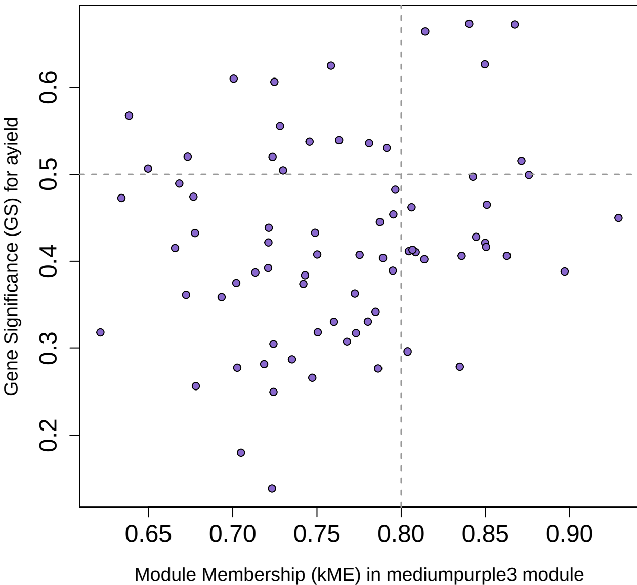
Membership vs. Significance mediumpurple3 module cor=0.18, p=0.12
