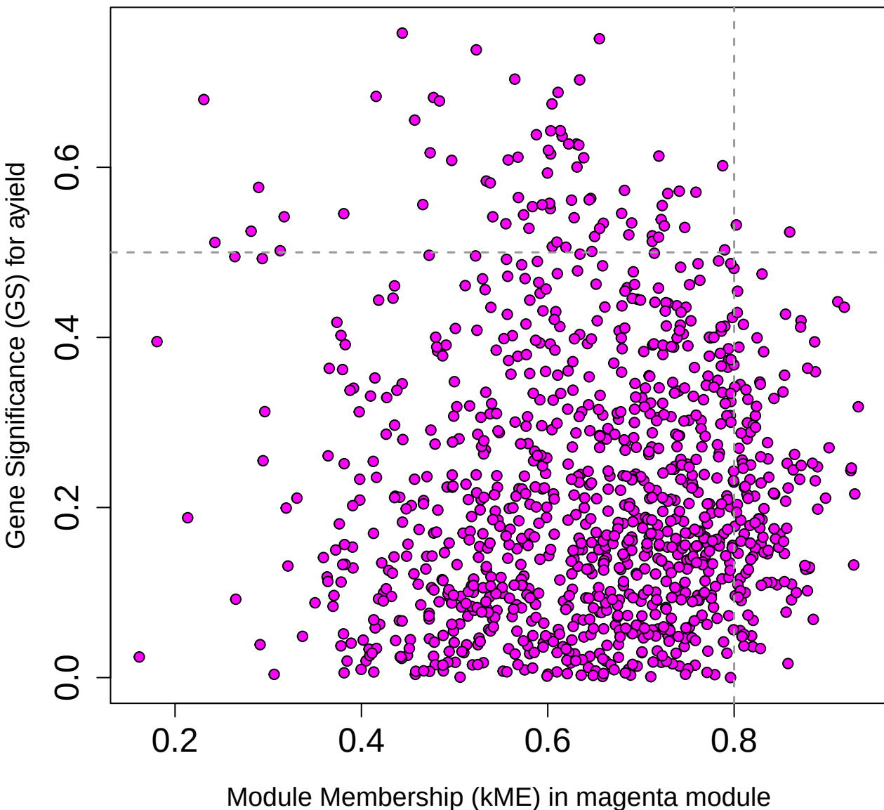
Membership vs. Significance magenta module cor=0.019, p=0.53
