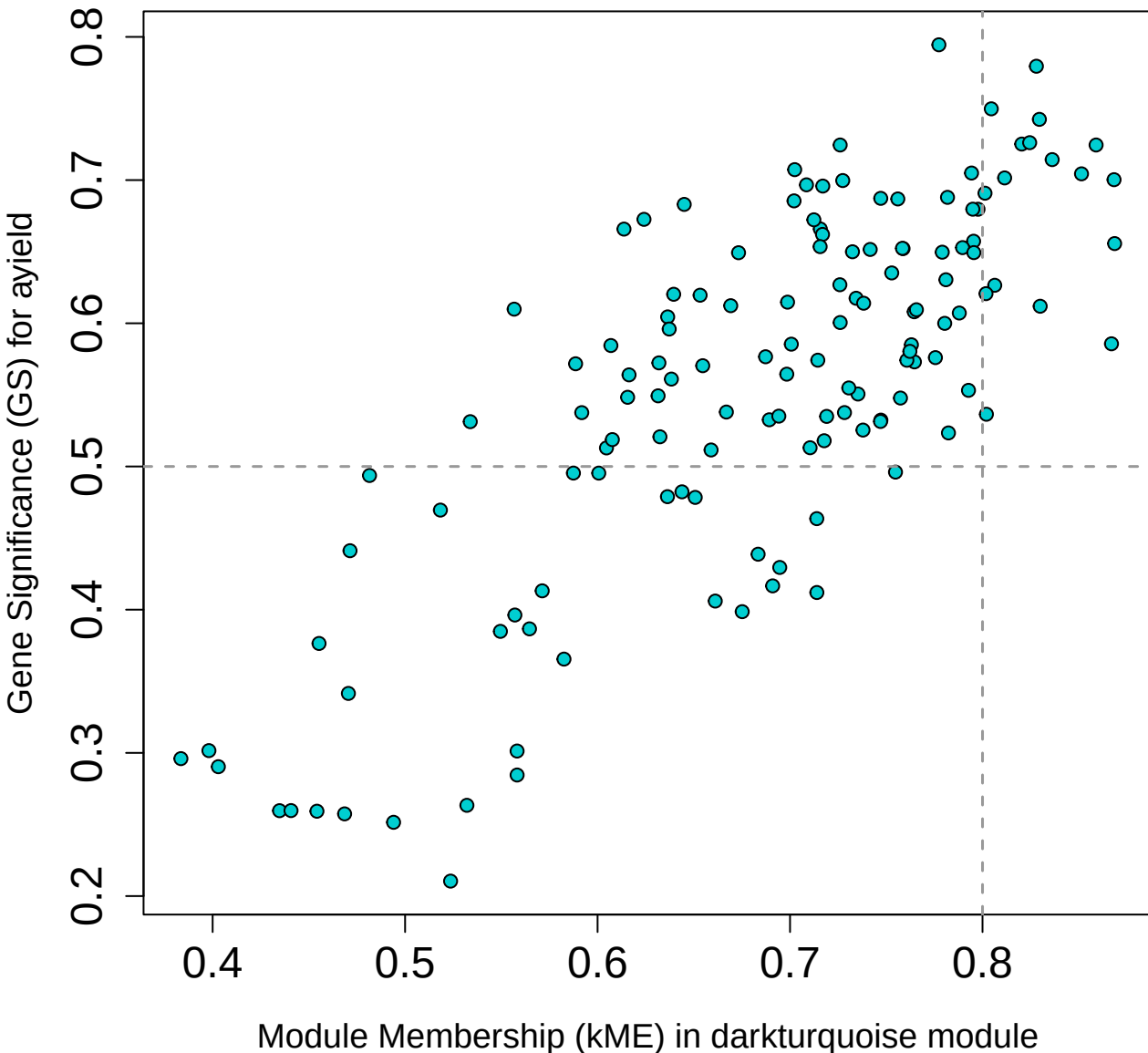
Membership vs. Significance darkturquoise module cor=0.78, p=4.6e-29
