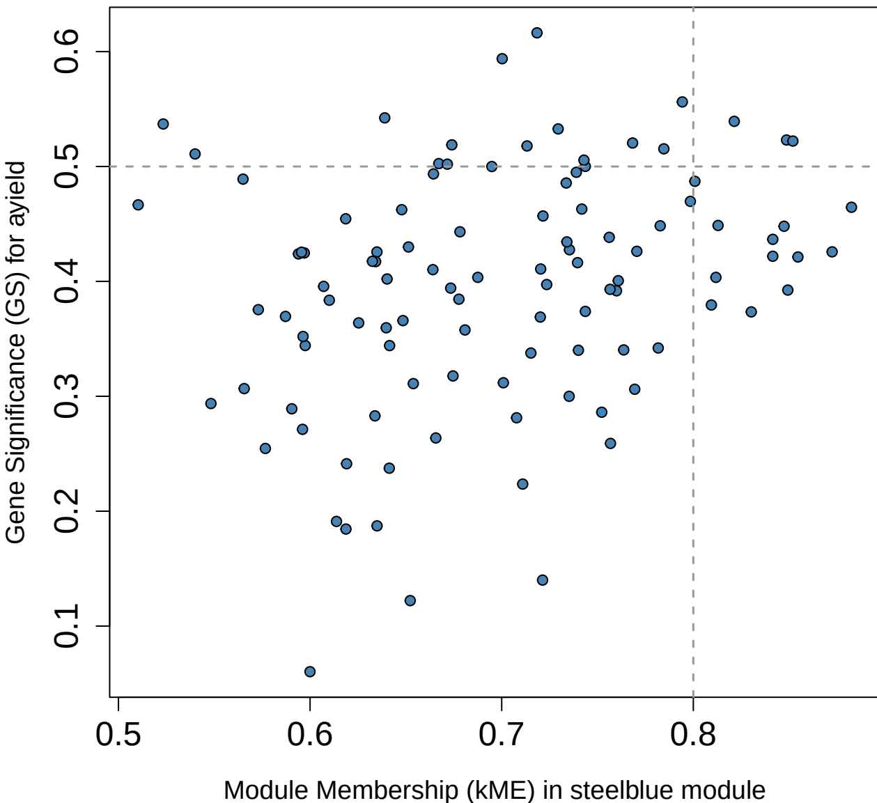
Membership vs. Significance steelblue module cor=0.27, p=0.0051
