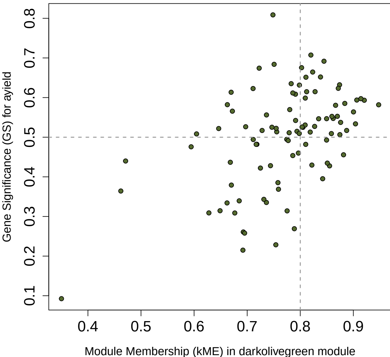
Membership vs. Significance darkolivegreen module cor=0.49, p=5.4e-07
