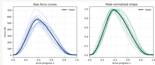
RP3 force curves -> sequence targets
