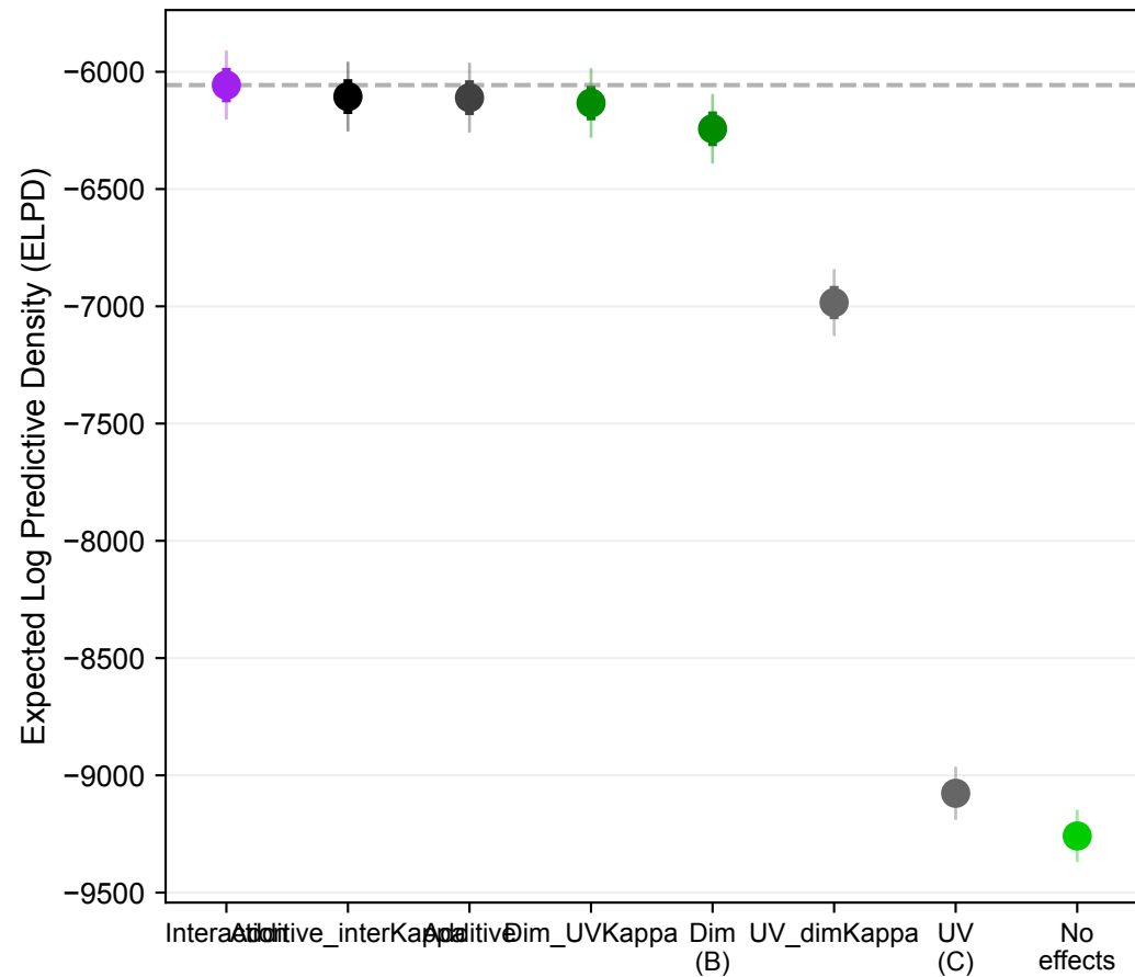
Absolute Model Performance
