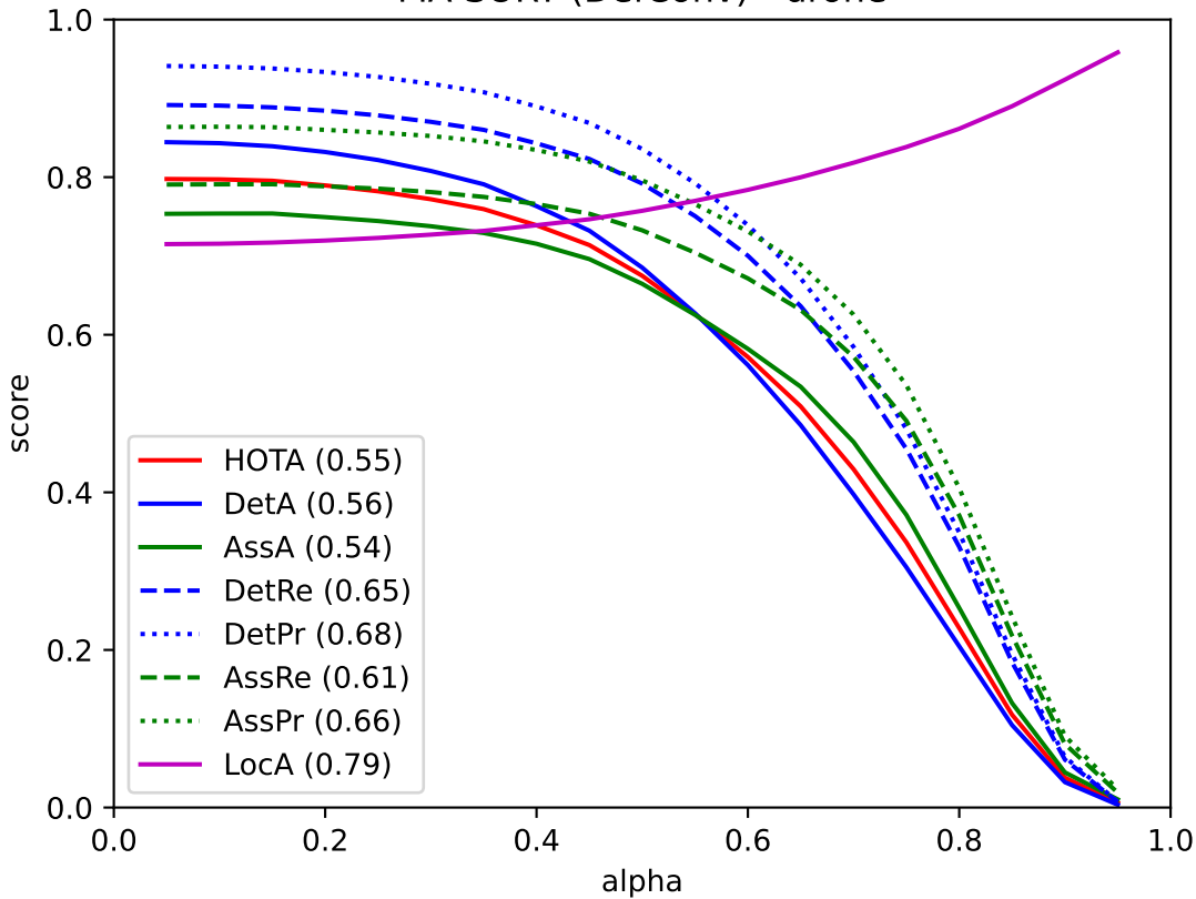
MA-SORT (DefConv) - drone
