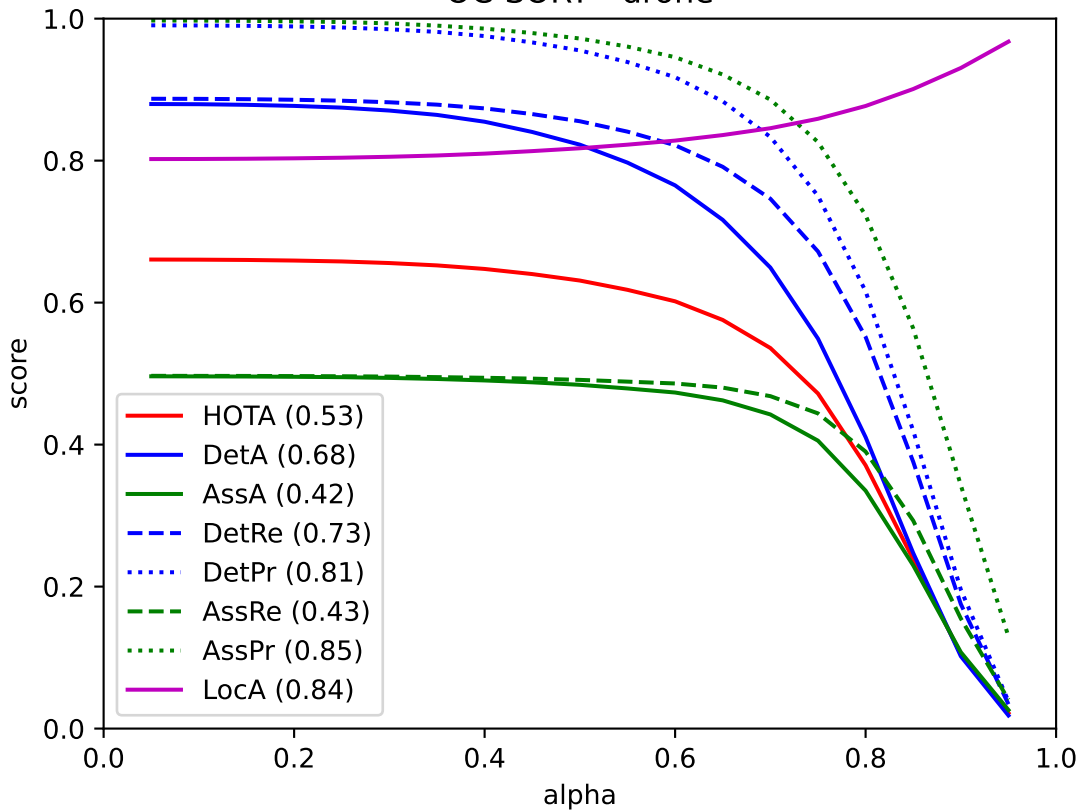
OC-SORT - drone
