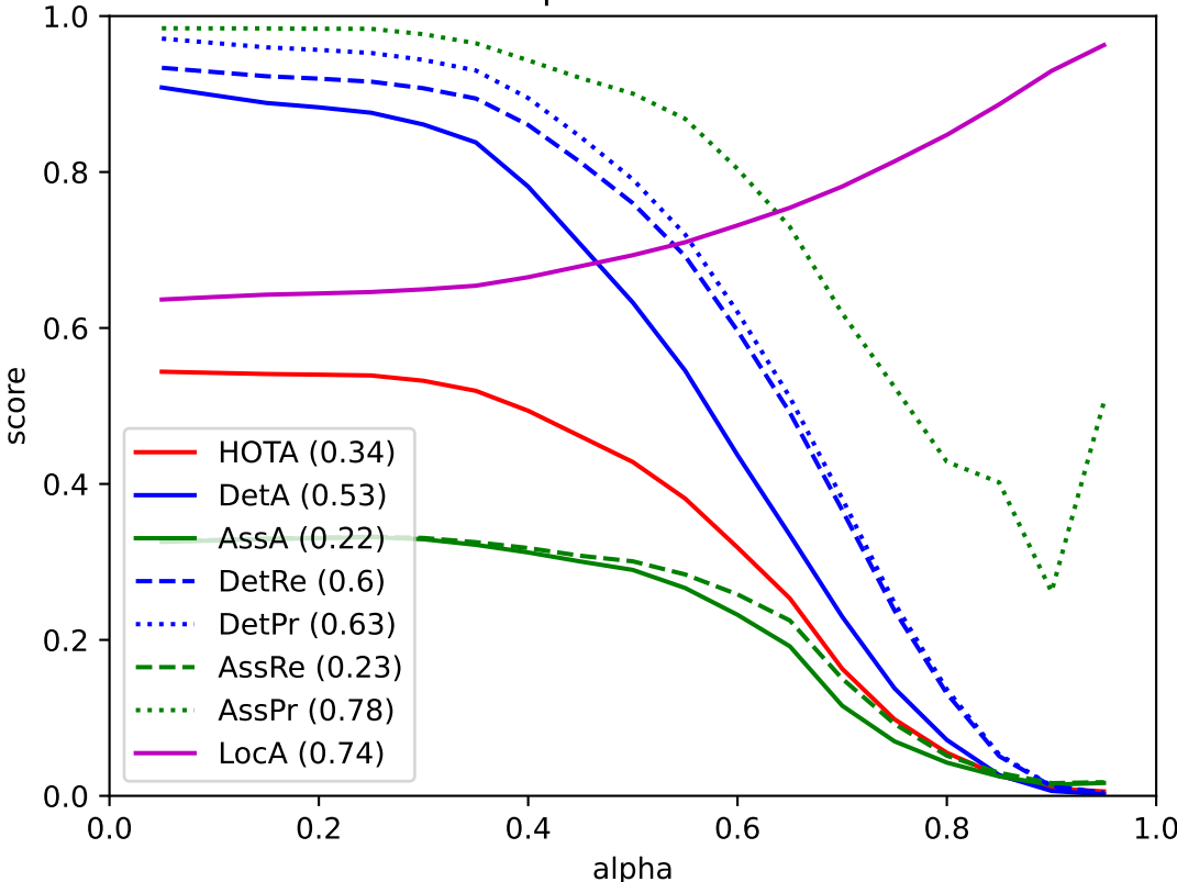
DeepSORT - drone
