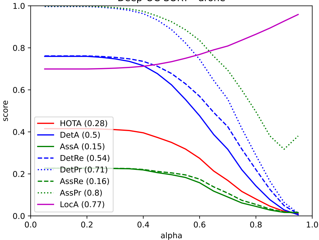
Deep-OC-SORT - drone
