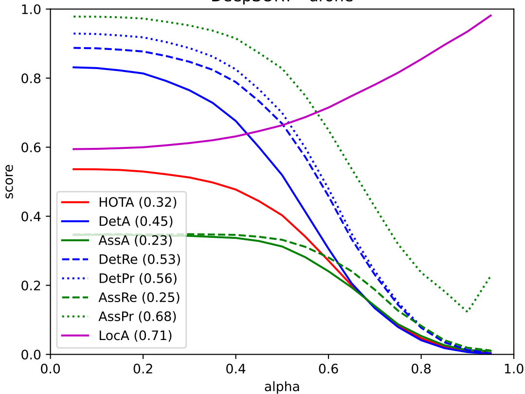
DeepSORT - drone
