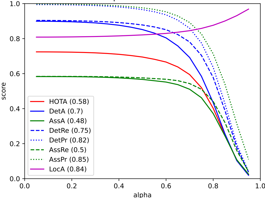
Deep-OC-SORT - drone
