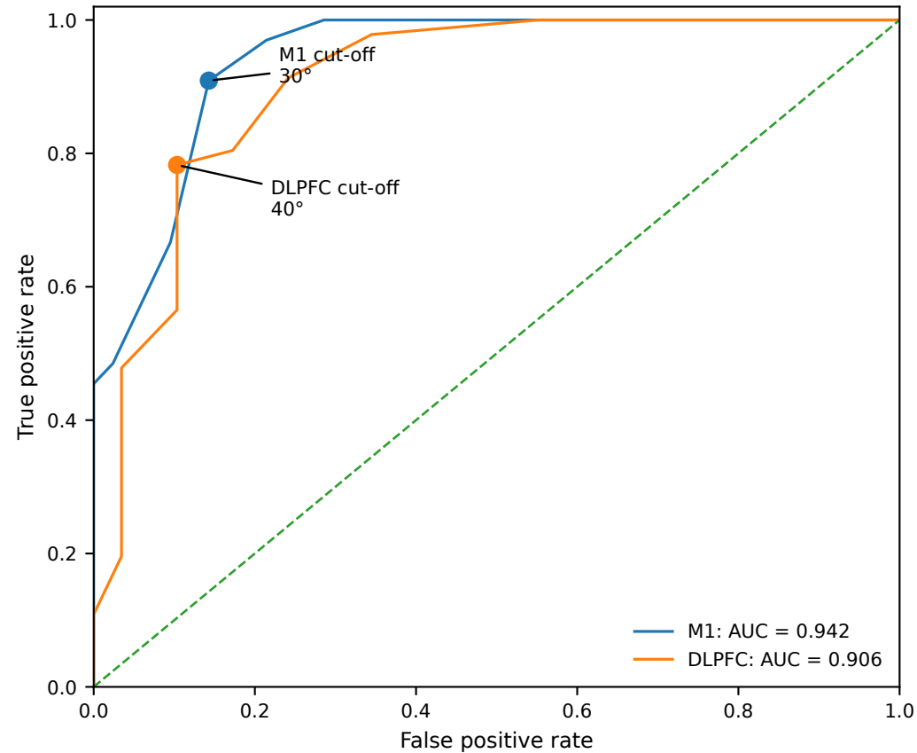
A. Clinical-to-optimal coil-yaw ROC
