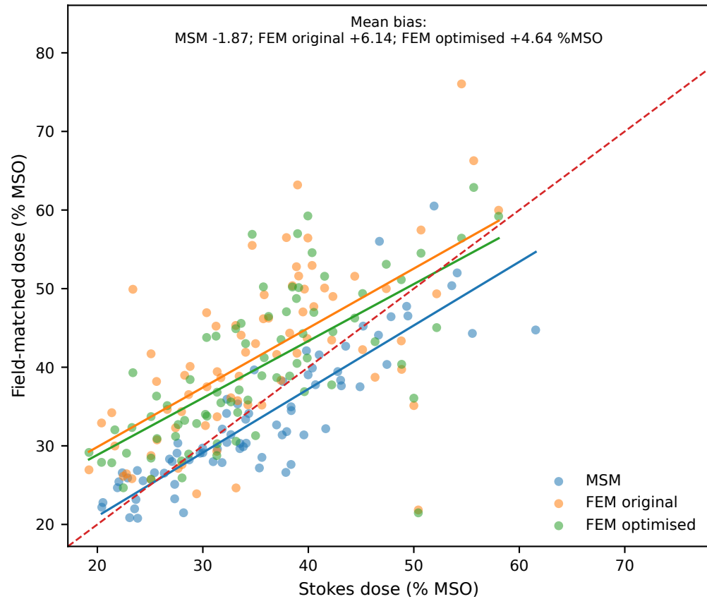
B. Stokes vs field-matched dose
