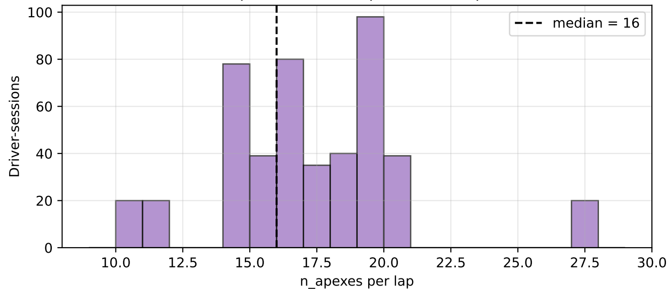
Apexes detected per fastest lap
