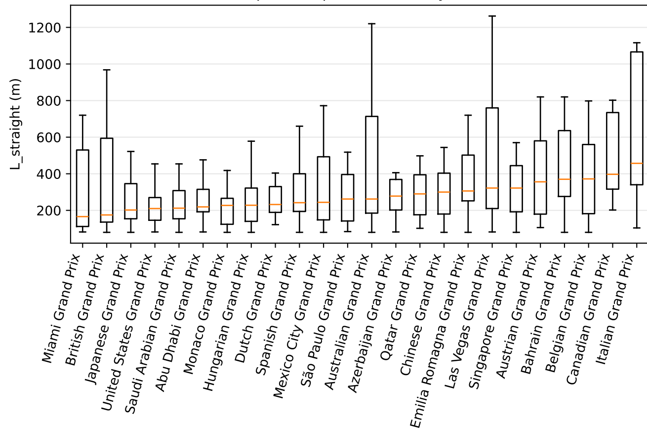
Apex-to-apex distance by GP
