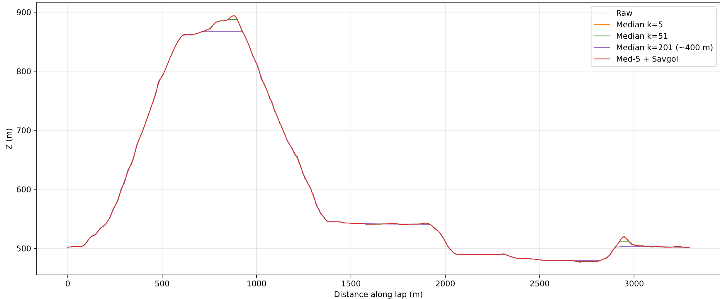
Monaco Z channel under increasing filter aggressiveness (real elevation differential ~32 m; none recover that)
