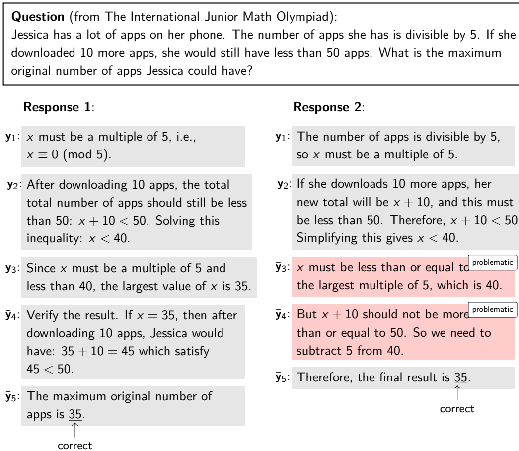
Fig. 4.11: Two LLM responses to a math problem. In response 1, both the final result and all the reasoning steps are correct. In response 2, the final result is correct, but there are mistakes in the reasoning process (highlighted in red). For outcome-based approaches, both responses are considered correct. For process-based approaches, the mistakes in response 2 can be considered in reward modeling.
