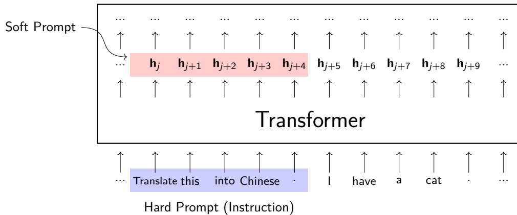
Fig. 3.3: Illustration of hard and soft prompts. Here the hard prompt is the instruction we input to the LLM for performing the task. The LLM encodes this instruction as usual, and the intermediate representations corresponding to the instruction can be viewed as some sort of soft prompt.
