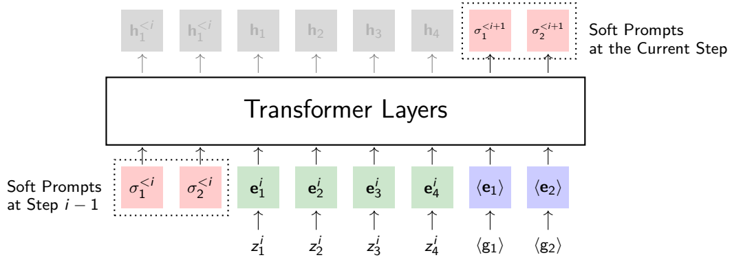
Fig. 3.8: Illustration of compressing a context segment into soft prompts ( \kappa = 2 and m_i = 4 ). The input to the LLM includes the soft prompts from the previous step ( \sigma_1^{<i> and \sigma_2^{<i> ), the tokens of the segment ( z_1, z_2, z_3 , and z_4 ), and the summary tokens ( \langle g_1 \rangle and \langle g_2 \rangle ). Given these, the LLM operates as usual. We then extract the outputs at the last Transformer layer that correspond to the summary tokens. These outputs can be viewed as the soft prompts that accumulated up to this segment.
