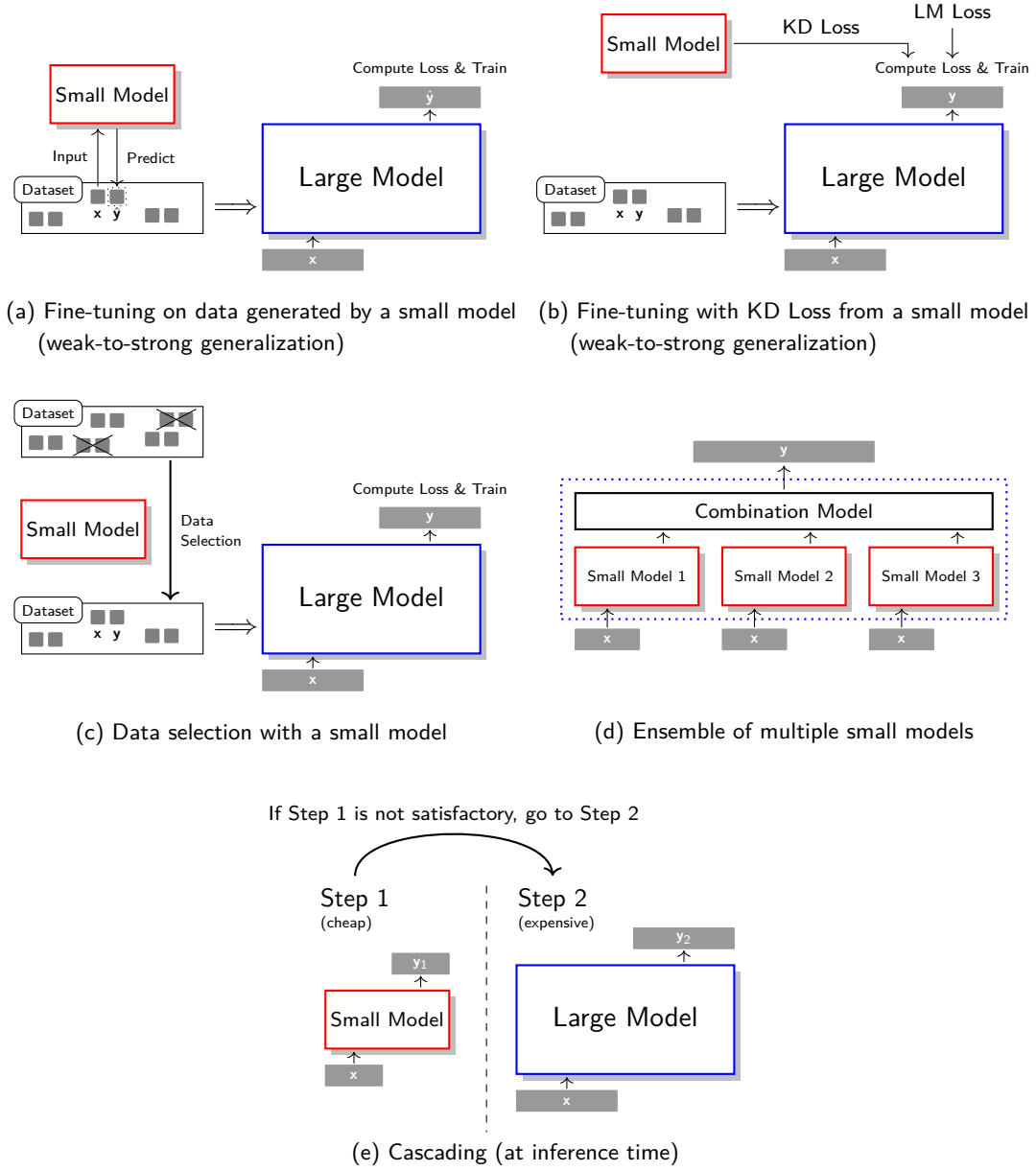
Fig. 4.5: Illustrations of using small models to improve large models in LLMs. One approach involves using smaller models for the fine-tuning or pre-training of larger models. This includes generating synthetic data (a), incorporating auxiliary loss (b), and selecting appropriate data (c). Another approach involves combining small models and large models. This includes learning a strong model by aggregating multiple small models (d), and cascading small models with large models (e).
