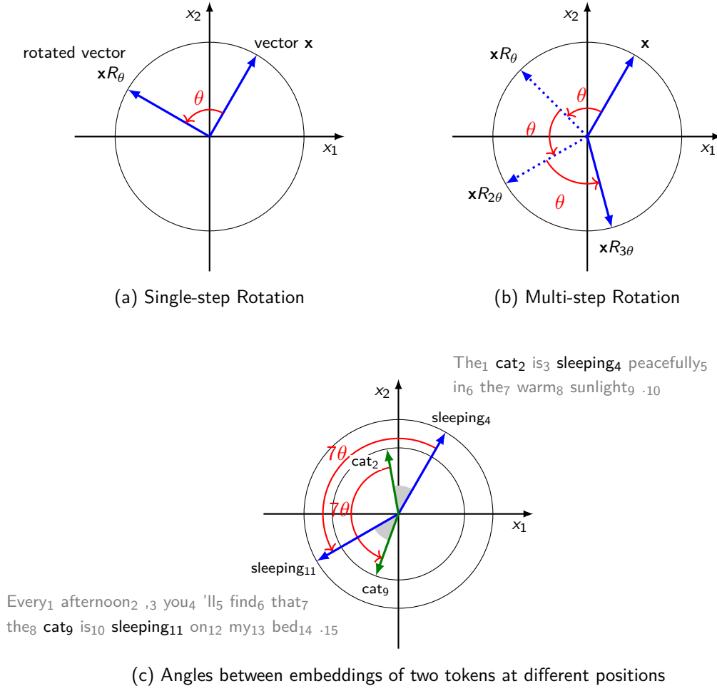
Fig. 2.12: Illustrations of vector rotations in a plane. Sub-figures (a) and (b) show rotations of a vector in a single step and multiple steps, respectively. Sub-figure (c) shows the embeddings of tokens cat and sleeping in two different sentences. We show these sentences with a subscript affixed to each token to indicate its position. If we represent tokens as vectors, we can add positional information by rotating these vectors. This rotation preserves the “distances” between the vectors. For example, given that the distance between cat and sleeping is the same in both sentences, the angle between their embeddings also remains the same during rotation.
