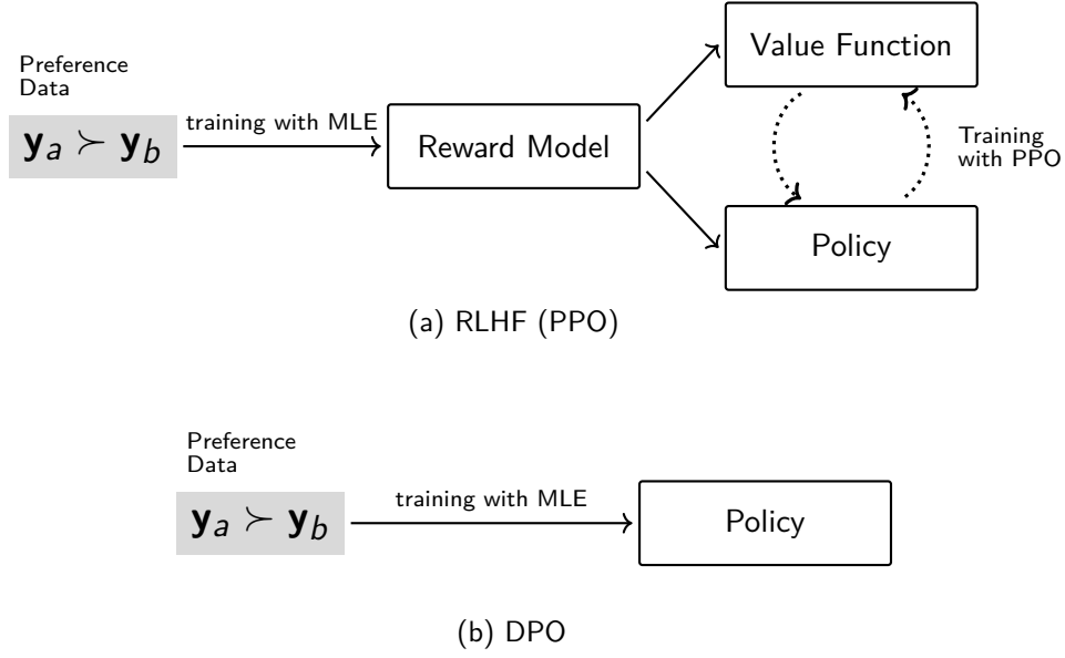
Fig. 4.10: Standard RLHF (PPO) vs. DPO. In RLHF, the human preference data is used to train a reward model, which is then employed in training the policy as well as the value function. In DPO, the use of human preference data is more direct, and the policy is trained on this data without the need for reward model training.
