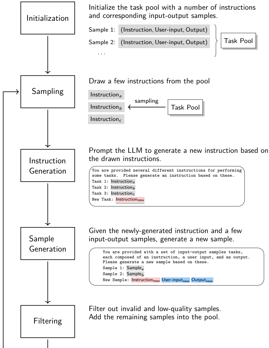
Fig. 4.4: Illustration of self-instruct [Wang et al., 2023b]. This method maintains a pool of instructions and corresponding input-output samples. Initially, the pool contains a number of hand-crafted instructions and samples. Each time, we draw a few instructions from the pool. An LLM is then prompted to generate new instructions and samples based on those drawn. Finally, the newly-generated instructions and samples are filtered and added to the pool.
