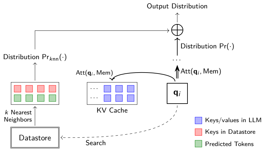
(b) k -NN Language Modeling
