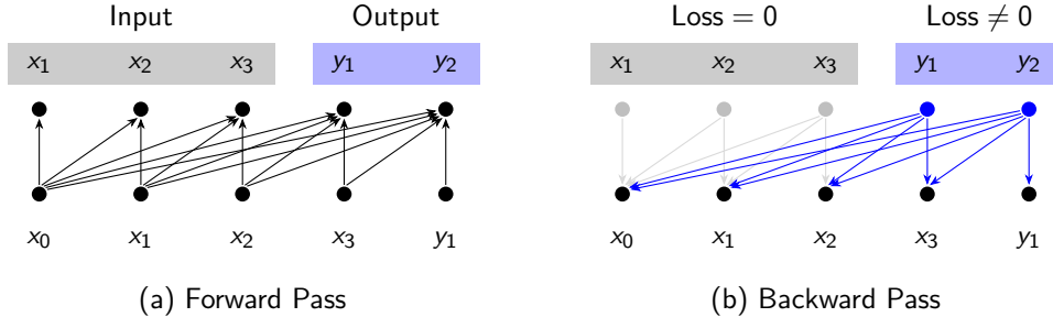
Fig. 4.2: Illustration of supervised fine-tuning for LLMs. We concatenate the input and the output into a single sequence. During the forward pass, we run the LLM as usual. During the backward pass, we compute the loss only for the output part and simply set the loss for the input part to 0.
