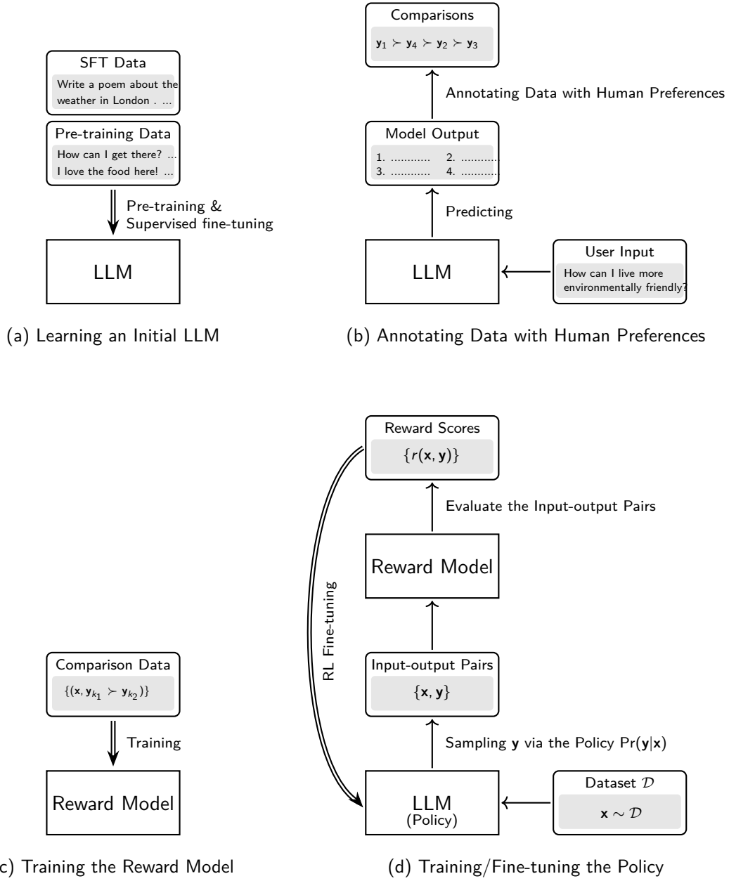
Fig. 2.2: An overview of RLHF. There are 4 key steps involved: a) training an initial LLM (i.e., policy) using pre-training and supervised fine-tuning; b) collecting human preference data by ranking the outputs of the LLM; c) training a reward model using the ranking results; d) RL fine-tuning of the policy based on the reward model. Double line arrows mean training or fine-tuning.
