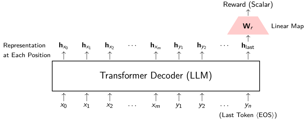
Fig. 4.8: Architecture of the reward model based on Transformer. The main component of this model is still an LLM. We use the Transformer decoder as the sequence representation model. We extract the representation of the last position of the decoder as the representation of the entire sequence [x, y] . We then map this representation to a scalar through a linear transformation, which serves as the reward score for [x, y] .
