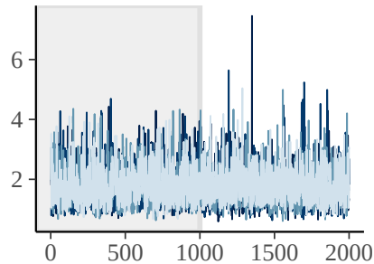
absorption rate
