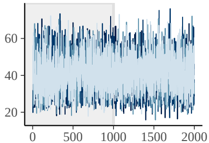
central compartment volume
