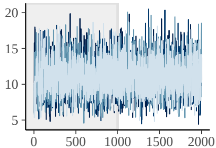
central clearance
