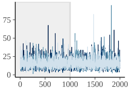
intercompartmental clearance
