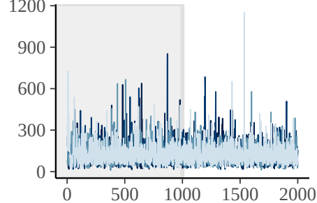
peripheral compartment volume
