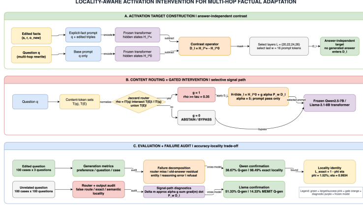
Fig. 1. Value-CQAG routes an edited context before prompt-only activation intervention. Edited and unrelated questions share the frozen model, while the evaluator measures both multi-hop answer quality and unchanged-output locality.
