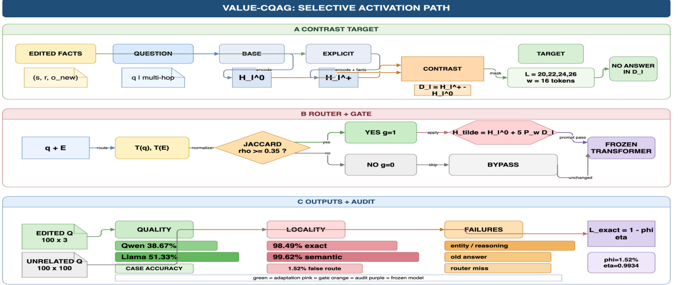
Fig. 1. Value-CQAG routes an edited context before prompt-only activation intervention. Edited and unrelated questions share the frozen model, while the evaluator measures both multi-hop answer quality and unchanged-output locality.
