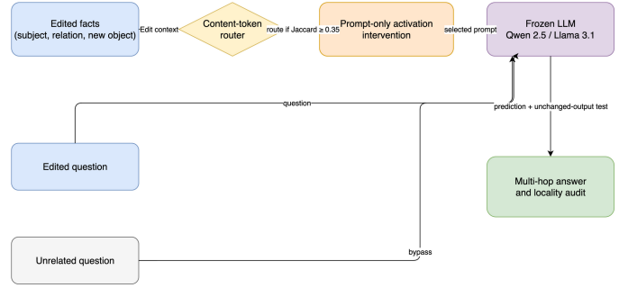
Fig. 1. Value-CQAG routes an edited context before prompt-only activation intervention. Edited and unrelated questions share the frozen model, while the evaluator measures both multi-hop answer quality and unchanged-output locality.
