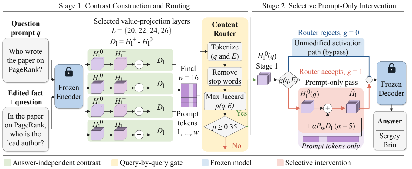
Fig. 1. Two-stage VALUE-CQAG pipeline (the layer labels illustrate the Qwen configuration; Llama uses {16, 20, 24, 28}). Stage 1 encodes question-only and edited-fact-conditioned prompts to obtain H_1^0(q) and H_1^+(q, \mathcal{E}) , while the router tests edit relevance. In Stage 2, rejected queries retain H_1^0(q) ; accepted queries receive the contrast D_1(q, \mathcal{E}) through \tilde{H}_1 before frozen decoding.
