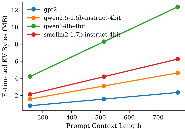
Context Length Tracks KV-Cache Traffic
