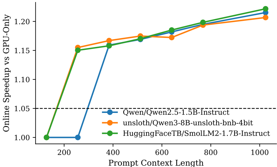
Dense Context Sweeps Reveal Regime Transition
