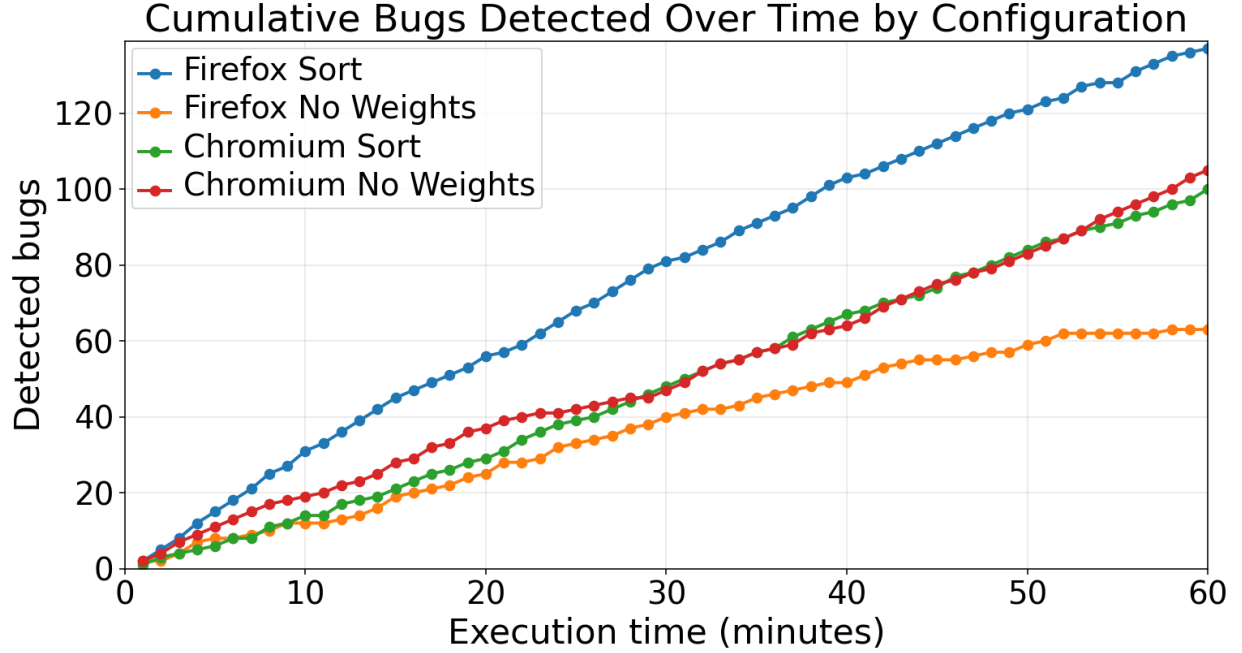
Figure 4: Cumulative bug reports for the weighted and no-weight configurations over the 60-minute evaluation window.
