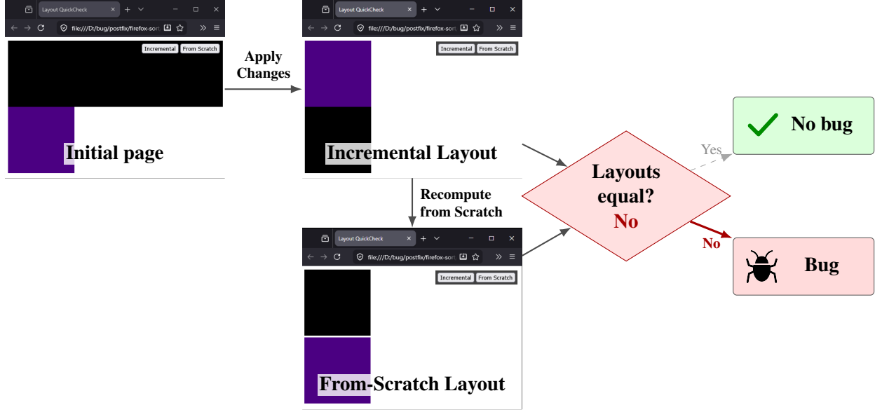
Figure 2: Example execution of the self-differential oracle. Starting from the initial page, LQC applies changes incrementally and recomputes the changed page from scratch. Different resulting layouts indicate an under-invalidation bug.
