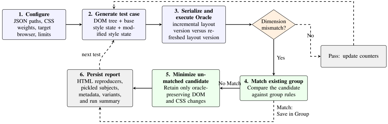
Figure 3: LQC pipeline. Each test case is tested by a layout oracle. Passing subjects advance the fuzzing loop; candidates are structurally classified, minimized when necessary, and persisted with their reproduction artifacts and cumulative metrics.
