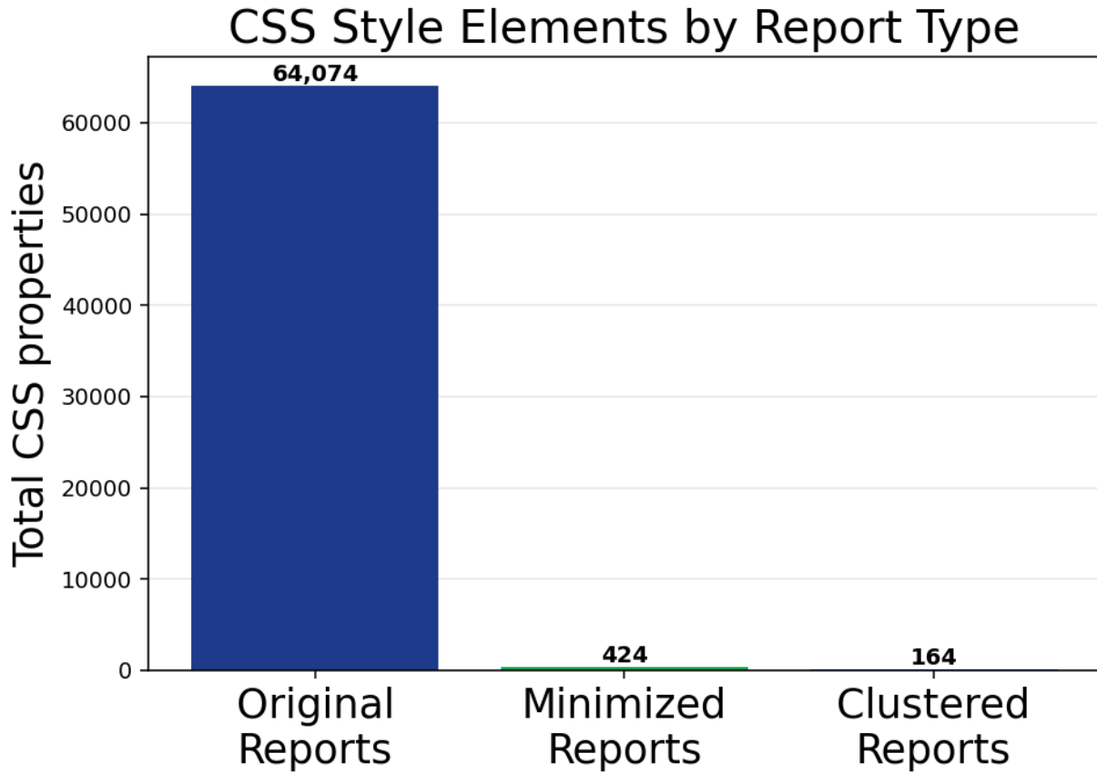
Figure 5: Total CSS style elements in grouped Firefox reports before minimization, after minimization, and after clustering.
