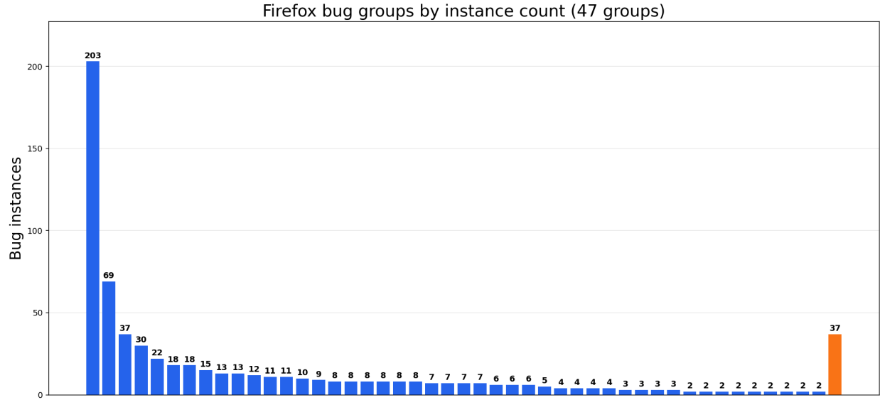
Figure 7: Firefox bug-group sizes, with all single bugs combined into one bar.
