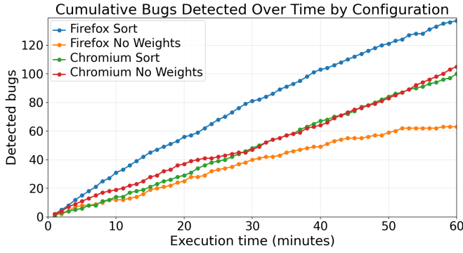
Fig. 5. Cumulative bug reports for the weighted and no-weight configurations over the 60-minute evaluation window.
