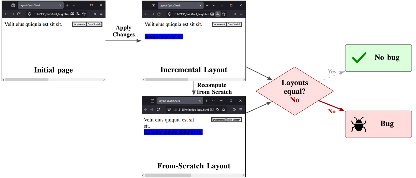
Fig. 3. Example execution of the self-differential oracle. Starting from the initial page, LQC applies changes incrementally and recomputes the changed page from scratch. Different resulting layouts indicate an under-invalidation bug.
