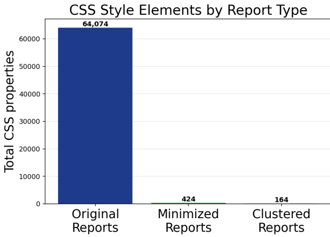
Fig. 6. Total CSS style elements in grouped Firefox reports before minimization, after minimization, and after clustering.
