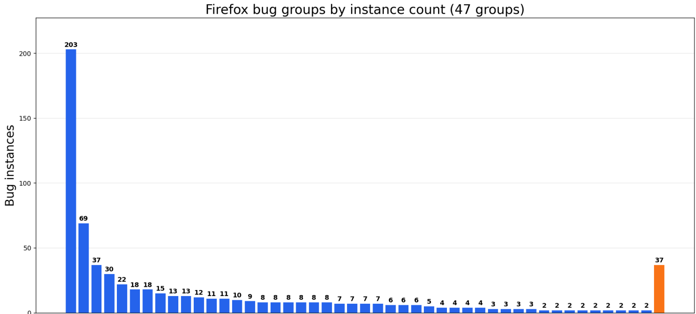
Fig. 8. Firefox bug-group sizes, with all single bugs combined into one bar.
