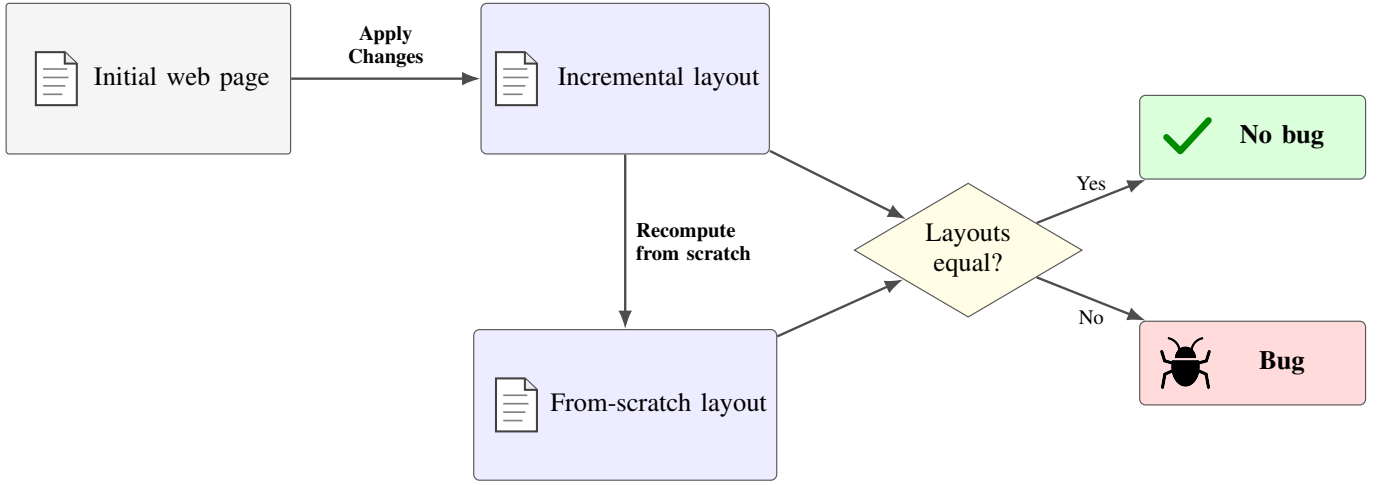
Fig. 2. LQC’s self-differential oracle compares incremental layout with layout computed from scratch for the same changed page. A difference indicates an under-invalidation bug.
