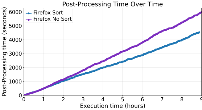
Fig. 7. Cumulative minimization and clustering time for Firefox sorting and no-sorting configurations.
