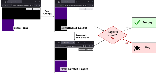
Fig. 2. Example execution of the self-differential oracle. Starting from the initial page, LQC applies changes incrementally and recomputes the changed page from scratch. Different resulting layouts indicate an under-invalidation bug.
