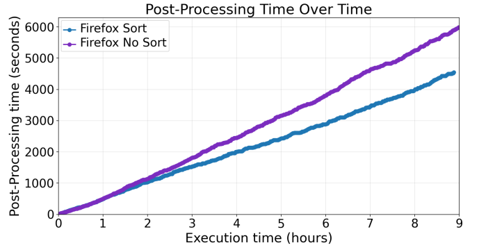
Fig. 6. Cumulative minimization and clustering time for Firefox sorting and no-sorting configurations.
