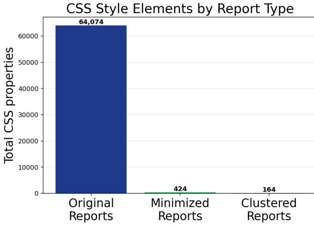
Fig. 5. Total CSS style elements in grouped Firefox reports before minimization, after minimization, and after clustering.
