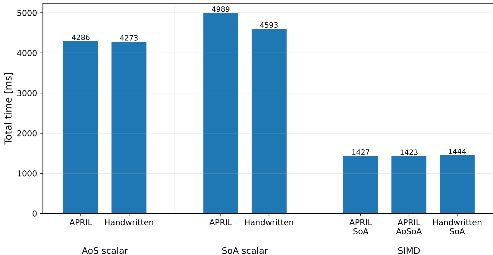
APRIL direct-sum benchmark vs handwritten kernels
