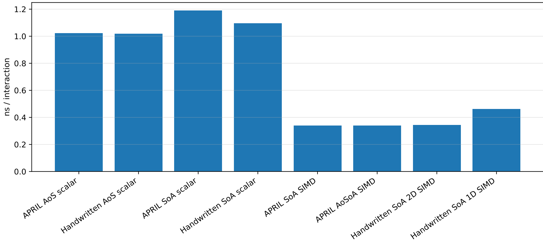
APRIL abstraction overhead vs handwritten kernels
