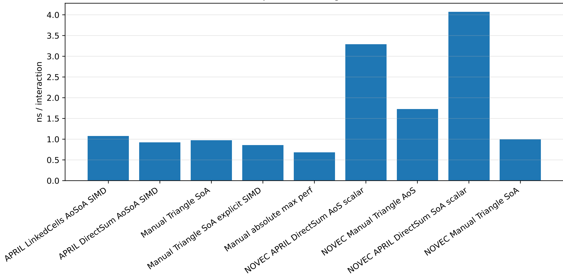
APRIL force-kernel performance against manual references
