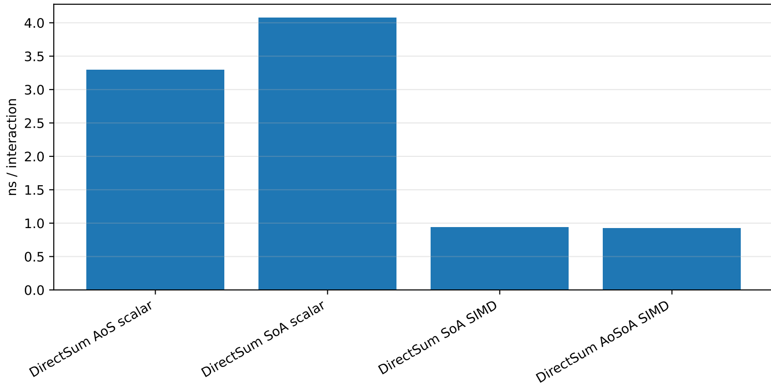
APRIL SIMD/layout impact: DirectSum
