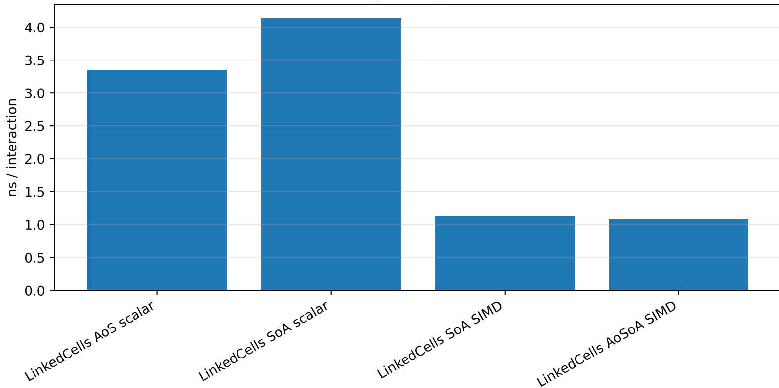
APRIL SIMD/layout impact: LinkedCells
