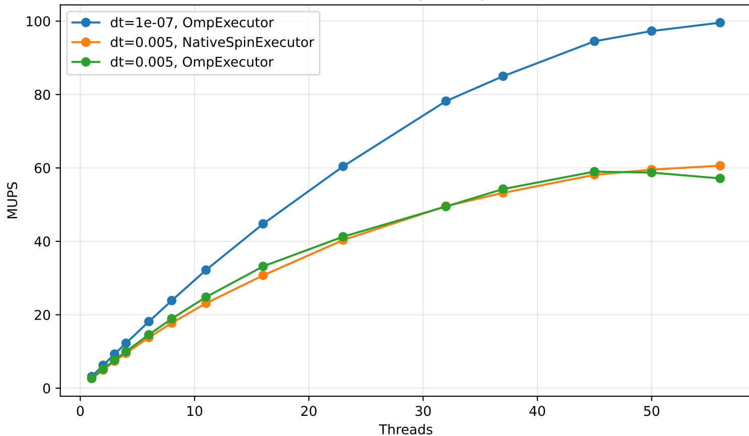
APRIL strong scaling
