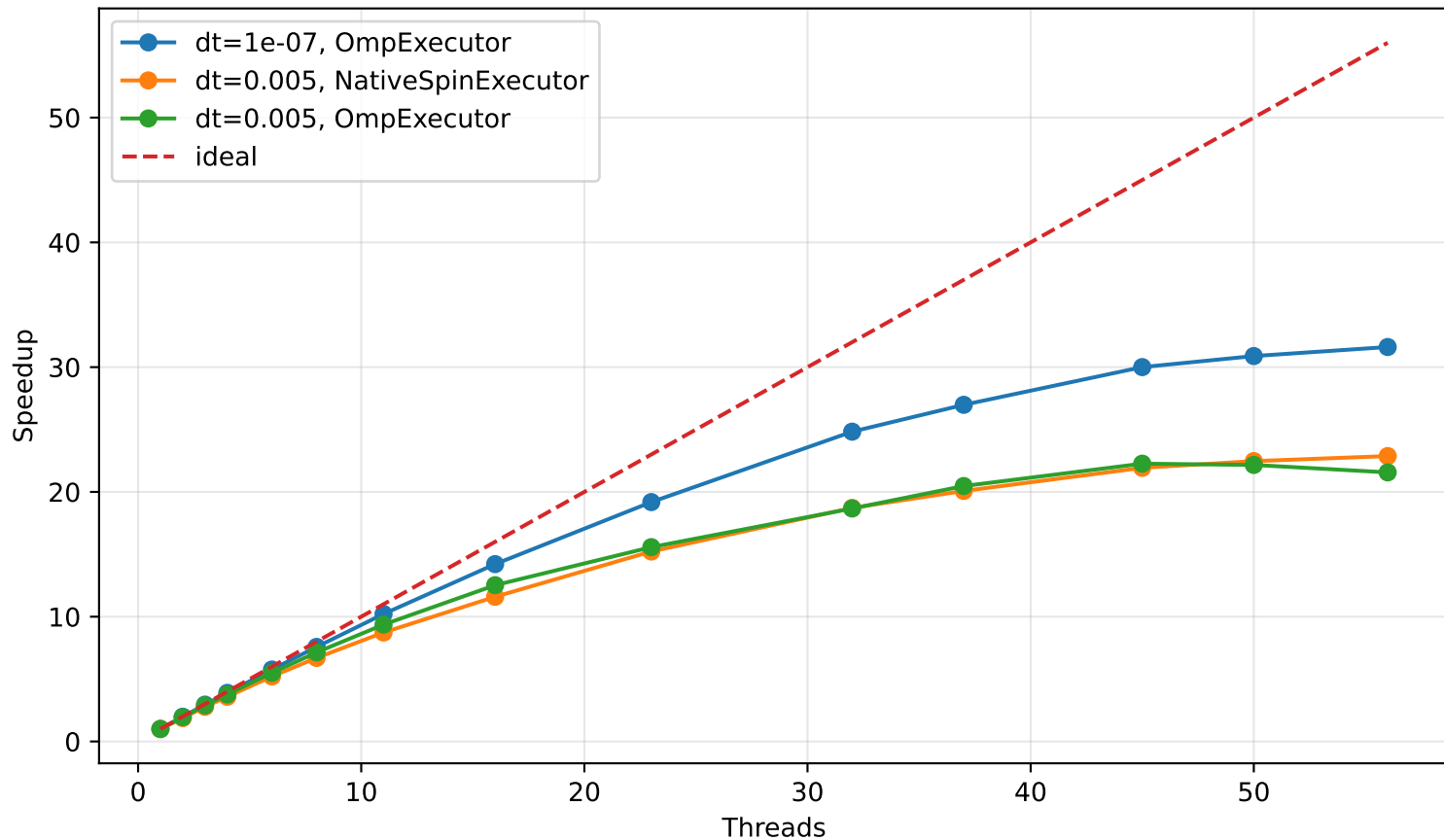
APRIL strong scaling speedup
