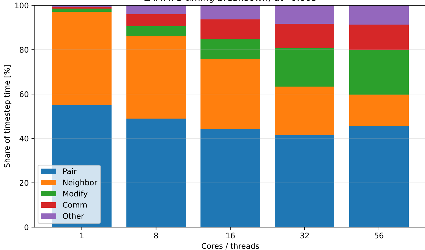
LAMMPS timing breakdown, dt=0.005
