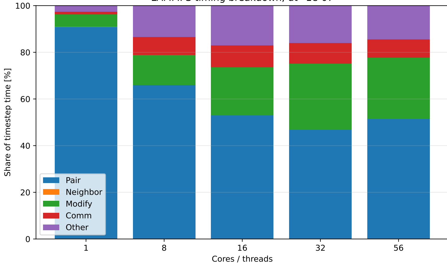
LAMMPS timing breakdown, dt=1e-07
