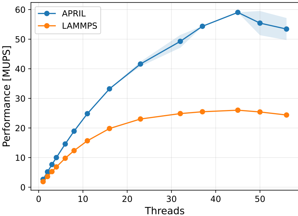
Throughput, \Delta t = 0.005
