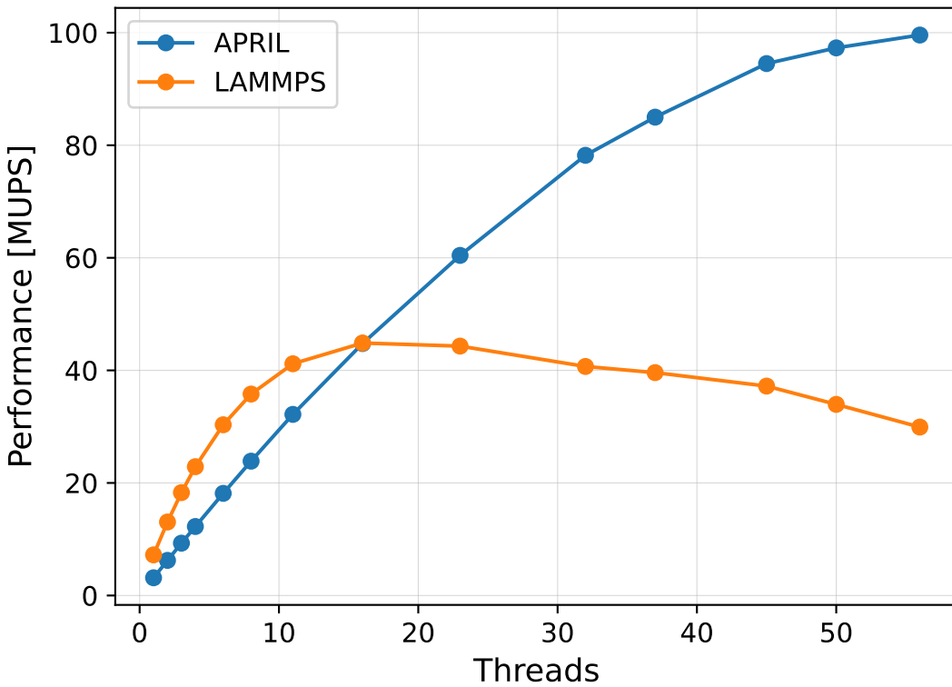
Throughput, \Delta t = 1e-07
