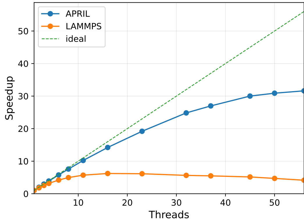
Strong scaling, \Delta t = 1e-07
