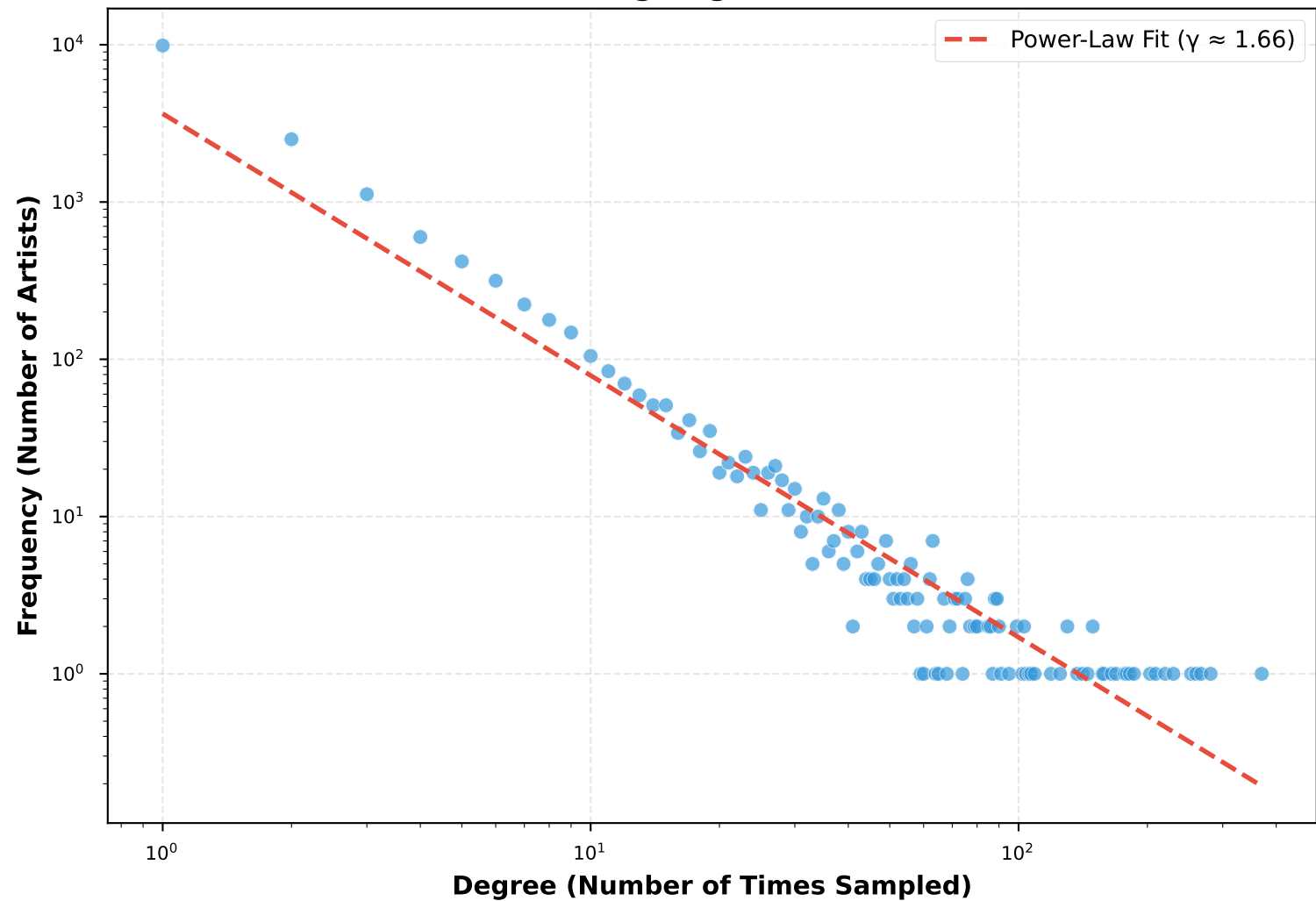
Degree Distribution of the Sampling Network (Log-Log Scale)
