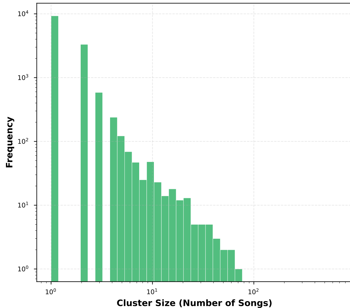
Cluster Size Distribution
