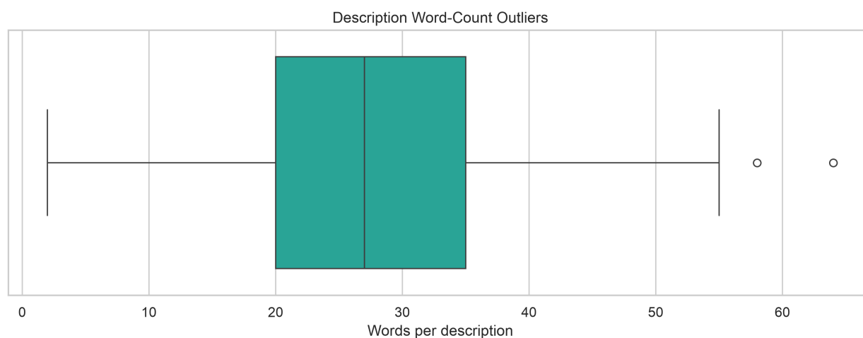
Figure 2. Long descriptions are valid observations; they are clipped rather than deleted.
