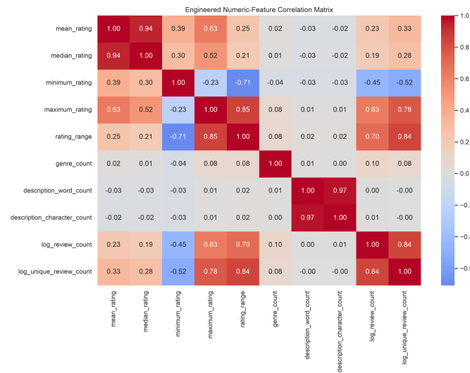
Figure 3. Length, rating, and popularity summaries contain redundancy, supporting feature reduction.
