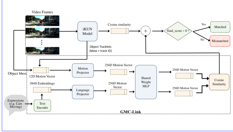
Fig. 1. The host model, iKUN in this case, provides tracking scores. The GMC-Link estimates camera motion, derives residual motion, aligns it with language, and provides an extra cue to adjust the tracking scores.
