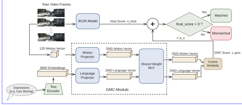
Fig. 1. The host model, iKUN in this case, provides tracking scores. The GMC-Link GMC Module estimates camera motion, derives residual motion, aligns it with language, and provides an extra cue to adjust the tracking scores.
