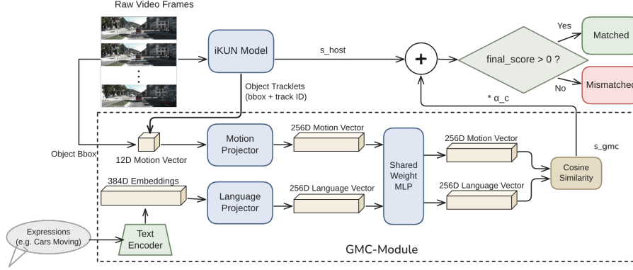
Fig. 1. The proposed RMOT framework with the global motion compensation module. The host model (iKUN in this case) provides tracking scores. The GMC Module estimates camera motion, derives residual motion, aligns it with language, and module provides an extra cue matching score to adjust the tracking scores matching results.
