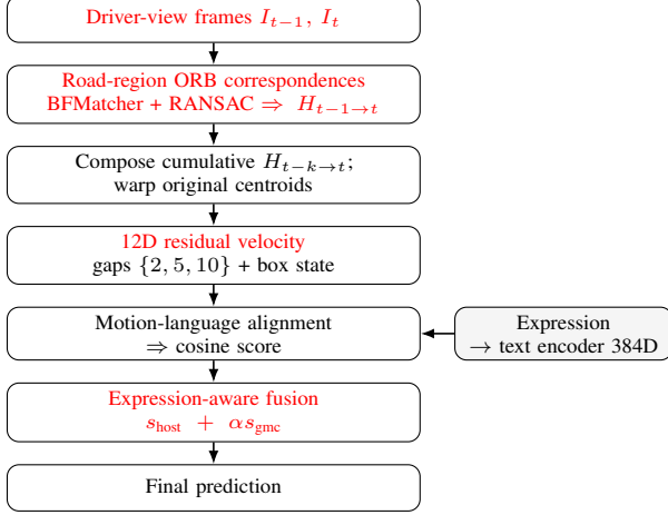
Fig. 2. GMC-Link pipeline. ORB homographies estimated from road-region features compose into a cumulative transform, produce a 12D residual-motion feature, align with the expression, and correct the host score through expression-aware late fusion.
