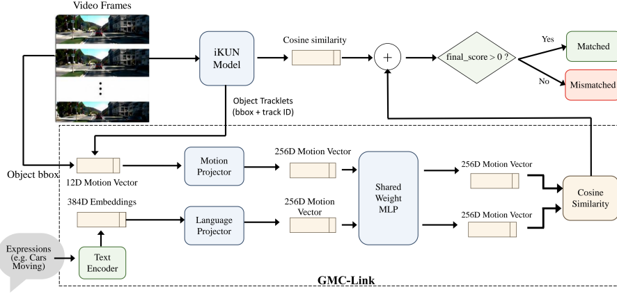
Fig. 1. The host model, iKUN in this case, provides tracking scores. The GMC-Link estimates camera motion, derives residual motion, aligns it with language, and provides an extra cue to adjust the tracking scores.
