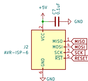
ISP connections for flashing / fuse changes
